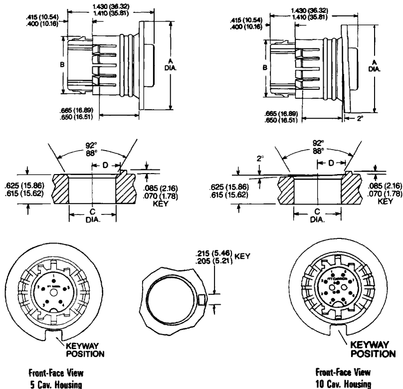
Snap-Thru Receptacle* (Mates with SLC-"P" Types)
