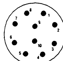
SLC-10 Face view, plug side
