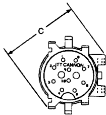
Front-Face View 10 Cavity Housing
