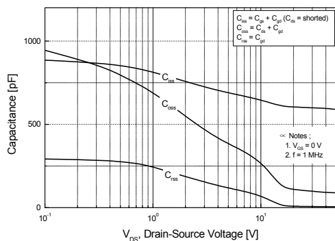
Figure 5. Capacitance Characteristics
