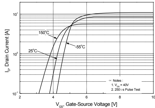
Figure 2. Transfer Characteristics
