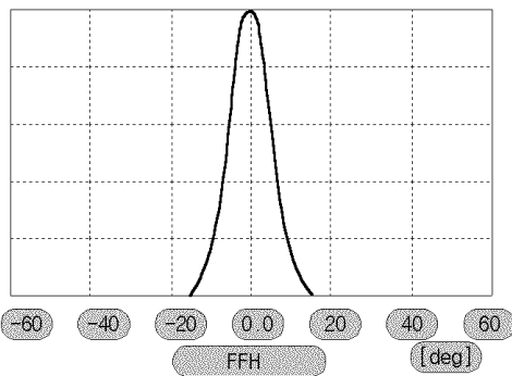
FAR-FIELD PATTERN FFH
