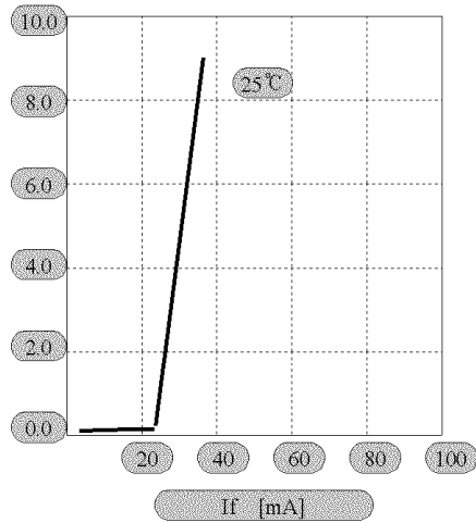
OPTICAL OUTPUT POWER vs CURRENT
