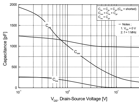
Figure 5. Capacitance Characteristics
