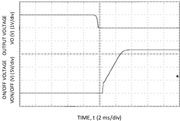
Start-up Using On/Off Voltage ( I_o = I_{o,max} ), V_o = 3.3V
