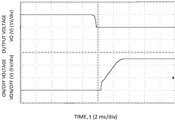
Start-up Using On/Off Voltage ( I_o = I_{o,max} ), V_o = 2.5V
