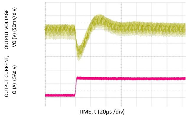
Transient Response to Dynamic Load Change from 50% to 100% at 12Vin, Cout=2x47uF, CTune=2200pF, RTune=300. Vo=5.0V
