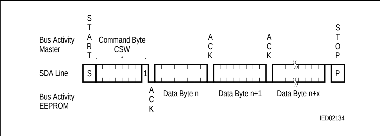
Figure 13 Sequential Read
