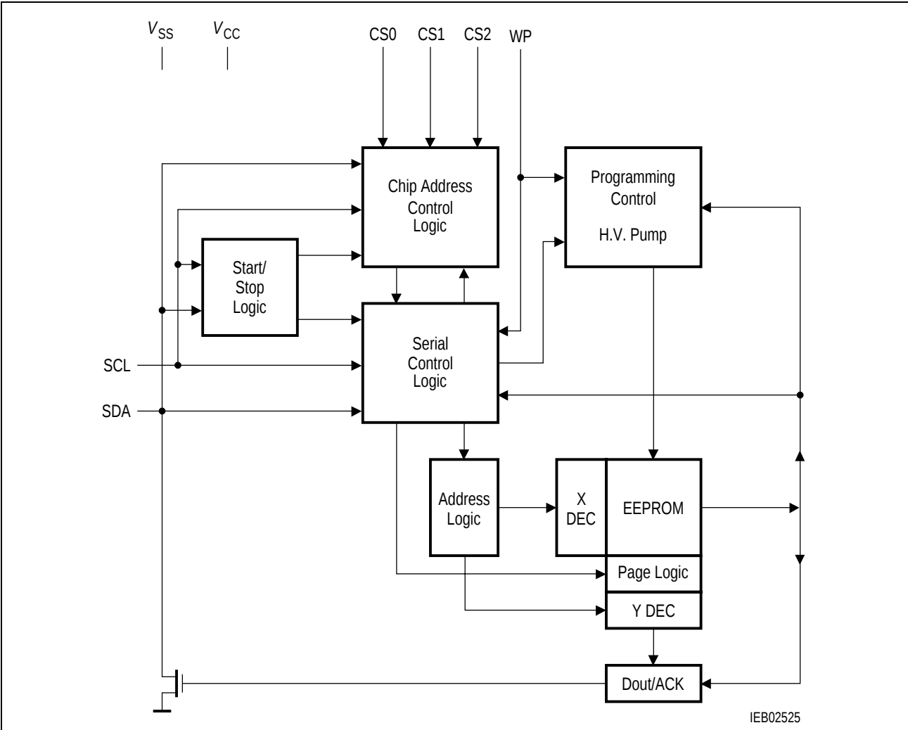
Figure 2 Block Diagram
