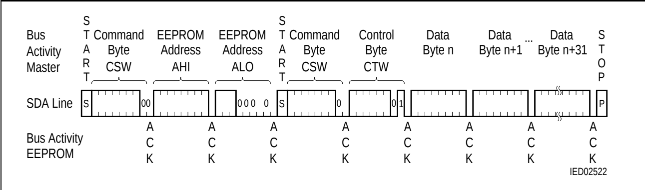
Figure 15 Sequence for Protection Bit Write
