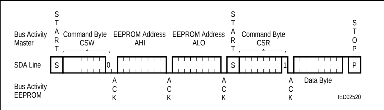
Figure 11 Random Read
