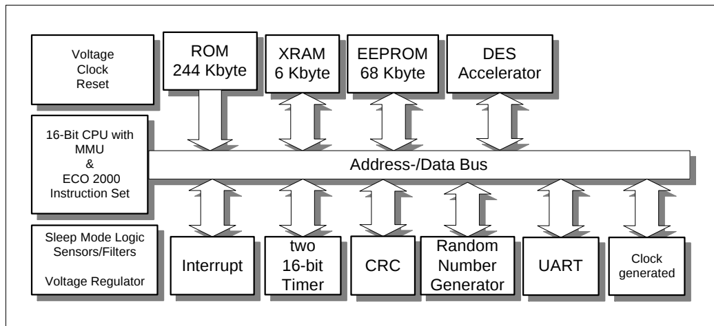
Figure 2: Block Diagram SLE 66C680PE
