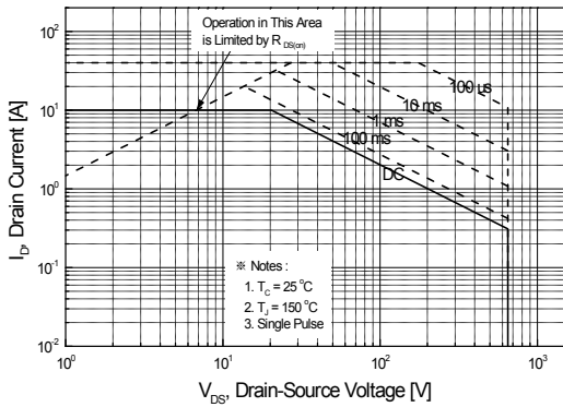
Figure 9-1. Maximum Safe Operating Area for SLP10N65C
