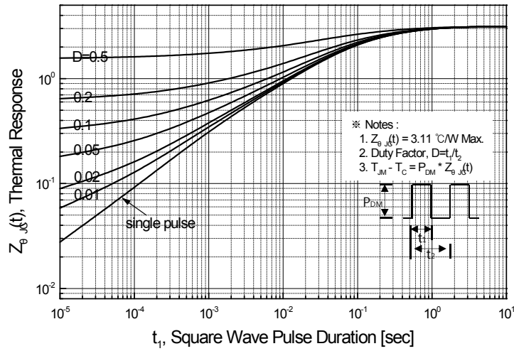
Figure 11-2. Transient Thermal Response Curve for SLF10N65C
