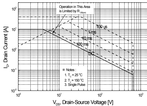
Figure 9-2. Maximum Safe Operating Area for SLF10N65C
