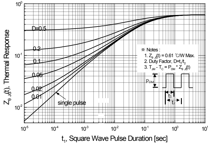
Figure 11-1. Transient Thermal Response Curve for SLP10N65C
