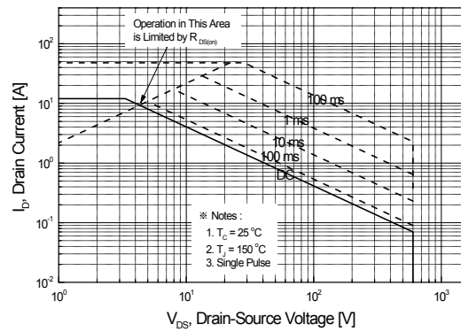
Figure 9-2. Maximum Safe Operating Area For SLF12N60UZ
