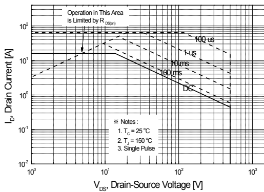
Figure 9-1. Maximum Safe Operating Area for SLP16N50C
