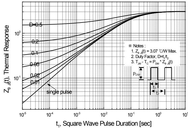
Figure 11-2. Transient Thermal Response Curve for SLF16N50C
