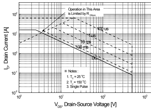
Figure 9-2. Maximum Safe Operating Area for SLF16N50C
