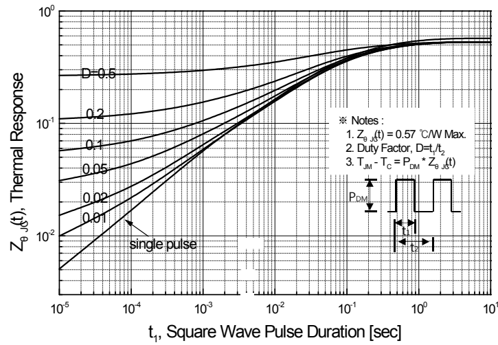
Figure 11-1. Transient Thermal Response Curve for SLP16N50C
