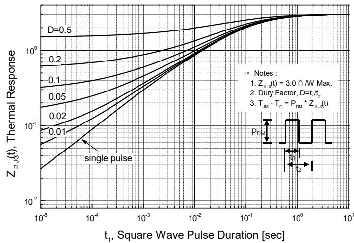
Figure 11-2. Transient Thermal Response Curve for SLF32N20C
