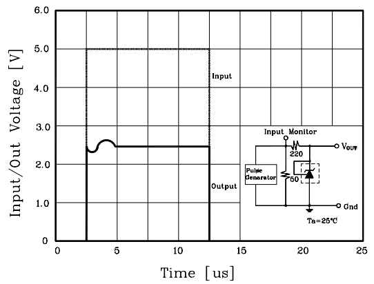
Fig. 9 Pulse reponse
