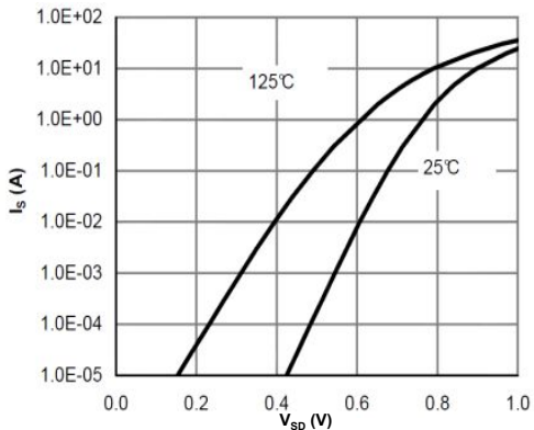
Figure 7: Body-Diode Characteristics
