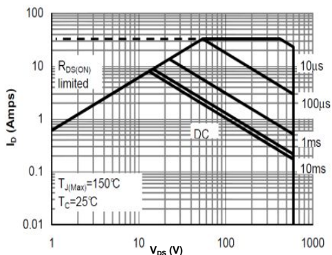
Figure 11: Maximum Forward Biased Safe Operating Area
