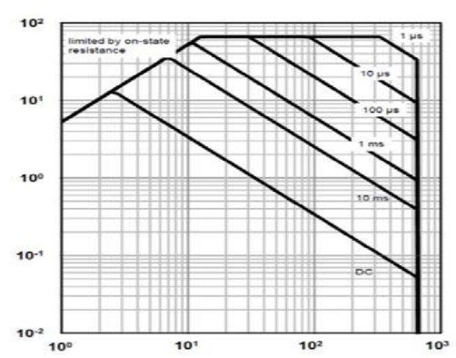
Figure 6. Maximum Safe Operating Area for SLF65R190SJ@25°C
