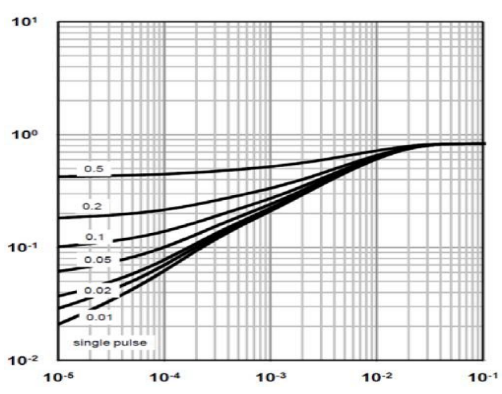
Figure 3. Transient Thermal Response Curve for SLP65R190SJ
