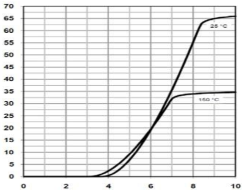
Figure 13. Transfer Characteristics
