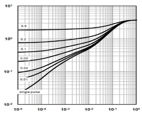
Figure 4. Transient Thermal Response Curve for SLF65R190SJ
