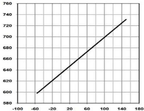
Figure 16. Breakdown Voltage Variation vs Temperature
