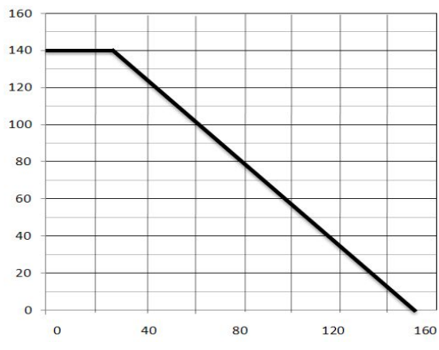
Figure 1. Power Dissipation for SLP65R190SJ
