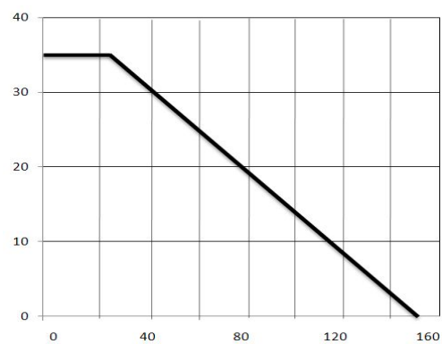
Figure 2. Power Dissipation for SLF65R190SJ
