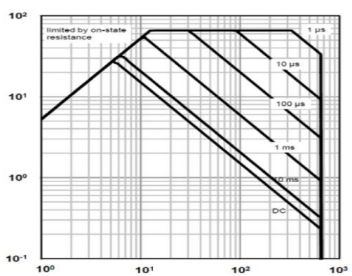
Figure 5. Maximum Safe Operating Area for SLP65R190SJ@25°C
