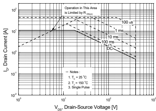
Figure 9-1. Maximum Safe Operating Area for SLP740UZ
