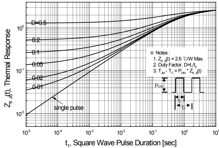
Figure 11-2. Transient Thermal Response Curve for SLF7N65C
