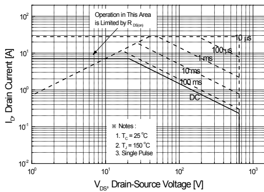
Figure 9-1. Maximum Safe Operating Area for SLP7N65C
