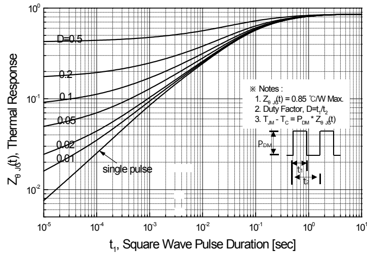
Figure 11-1. Transient Thermal Response Curve for SLP7N65C
