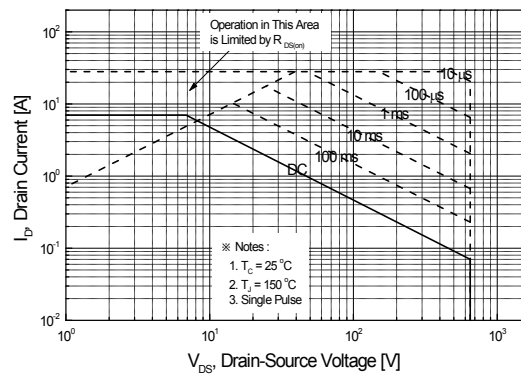
Figure 9-2. Maximum Safe Operating Area for SLF7N65C
