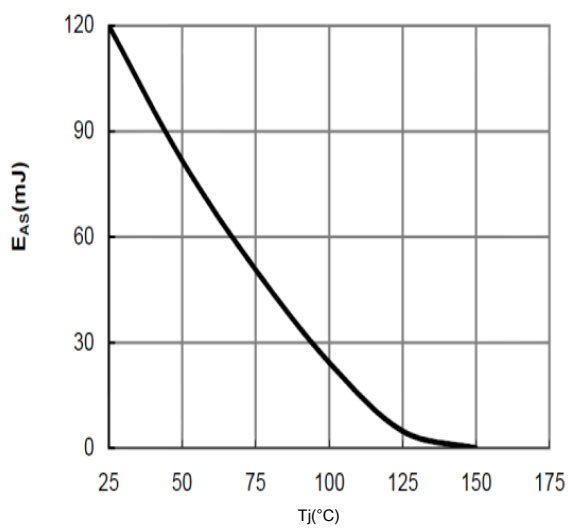
Figure 17: Avalanche energy
