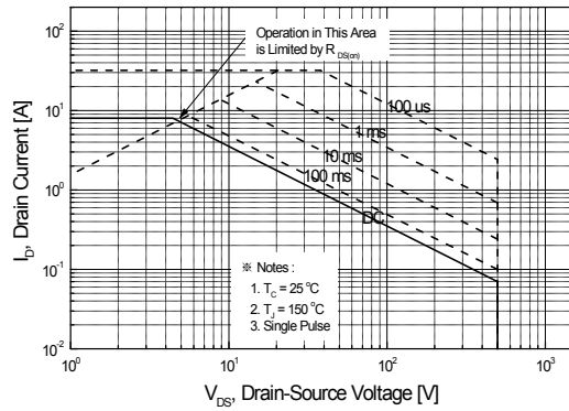
Figure 9-2. Maximum Safe Operating Area for SLF840C
