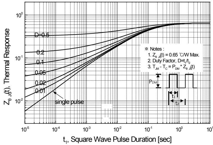
Figure 11-1. Transient Thermal Response Curve for SLP8N60C
