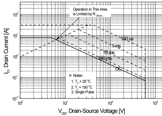
Figure 9-2. Maximum Safe Operating Area for SLF8N60C
