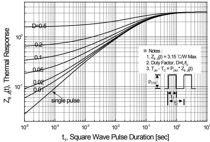
Figure 11-2. Transient Thermal Response Curve for SLF8N60C
