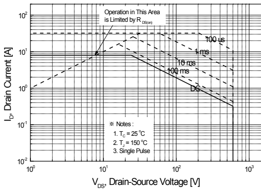
Figure 9-1. Maximum Safe Operating Area for SLP8N60C
