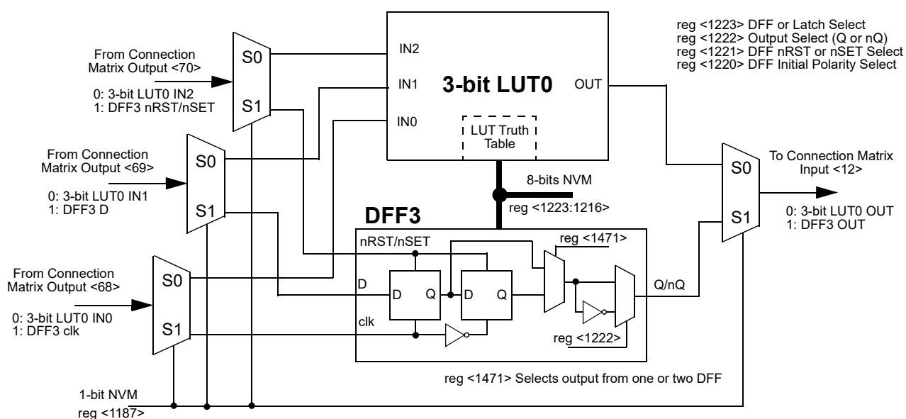
Figure 14. 3-bit LUT0 or DFF3 with RST/SET
