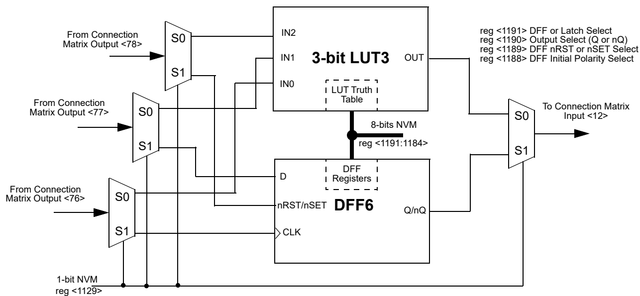
Figure 15. 3-bit LUT3 or DFF6
