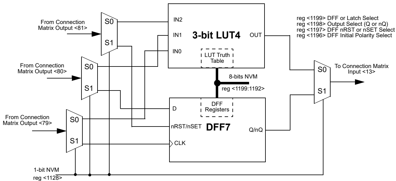
Figure 16. 3-bit LUT4 or DFF7
