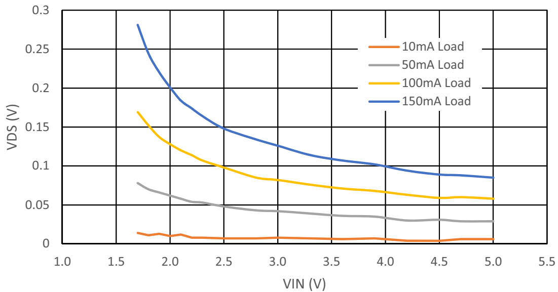
Figure 97. SLG46580 LDO Dropout Voltage vs. V_{IN}
