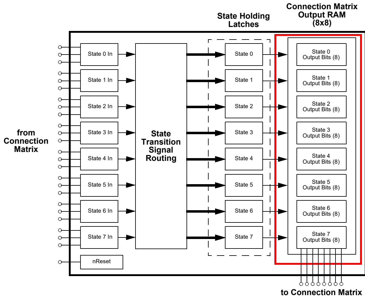
Figure 66. Connection Matrix Output RAM
