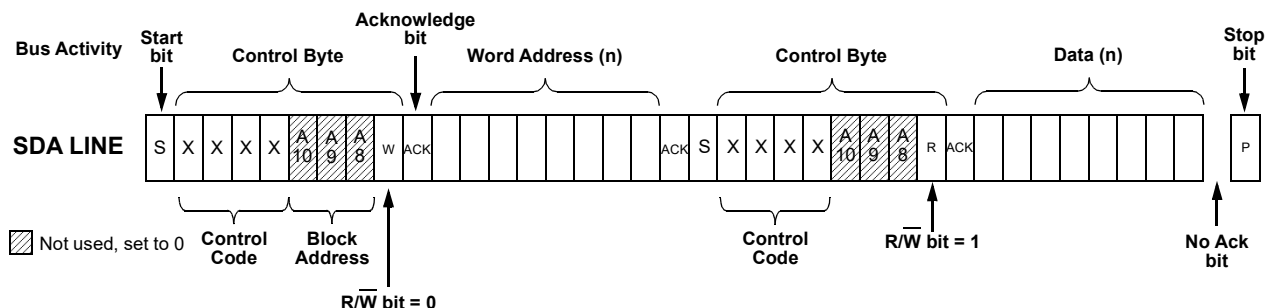
Figure 87. Random Read Command
