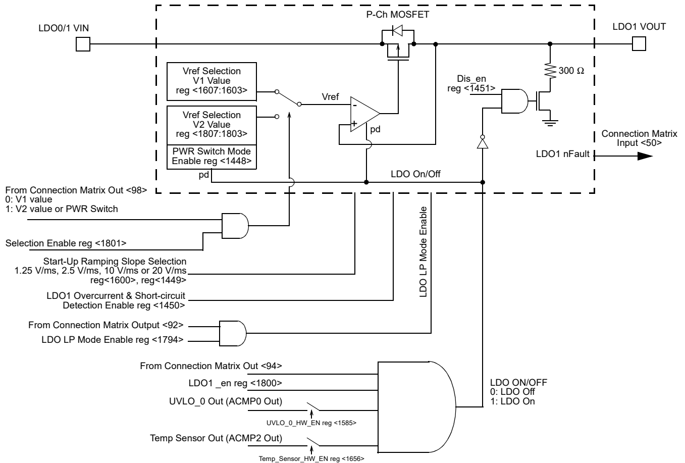
Figure 91. LDO1 Regulator Block Diagram
