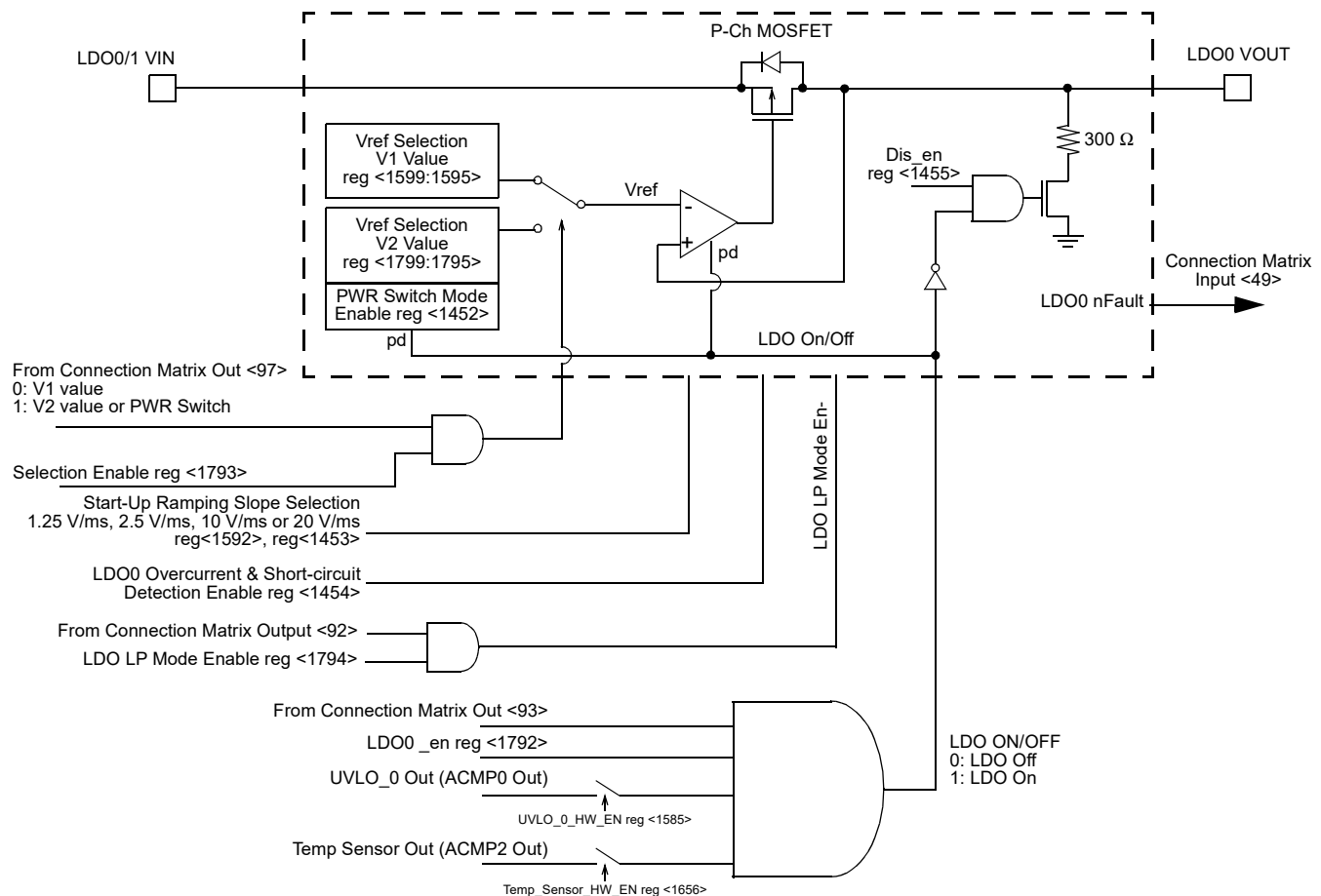
Figure 90. LDO0 Regulator Block Diagram
