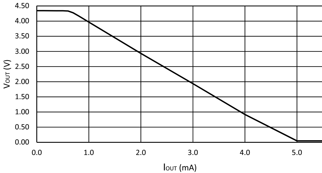
Figure 96. SLG46580 LDO Load Regulation, LOW POWER Mode, T = 25^{\circ}\text{C} , V_{DD} = 5\text{V} , V_{OUT} = 4.35\text{V}
