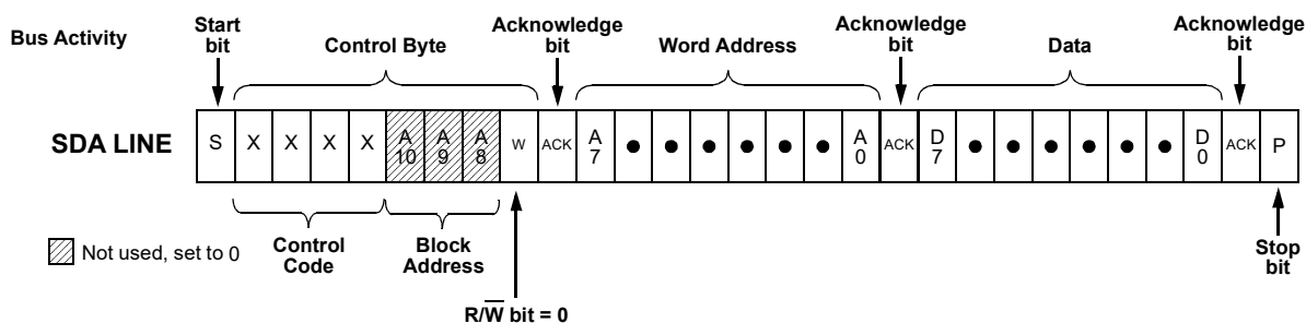
Figure 84. Byte Write Command, \overline{R/\overline{W}} = 0
