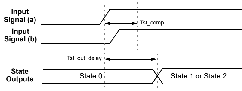
Figure 74. State Transition Timing - Competing Inputs Indeterminate
