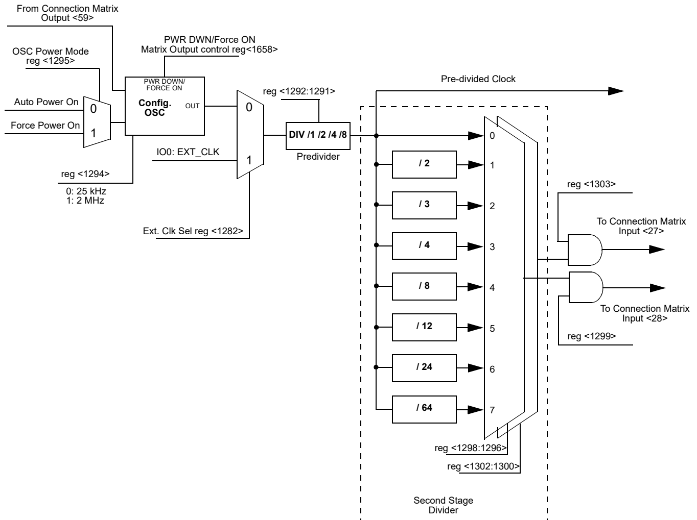
Figure 49. Configurable OSC Block Diagram
