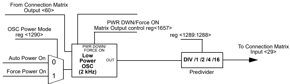
Figure 48. Low Power Oscillator Block Diagram
