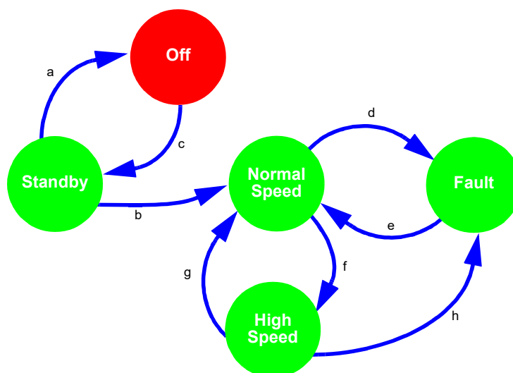
Figure 60. Asynchronous State Machine States and Transitions Diagram
