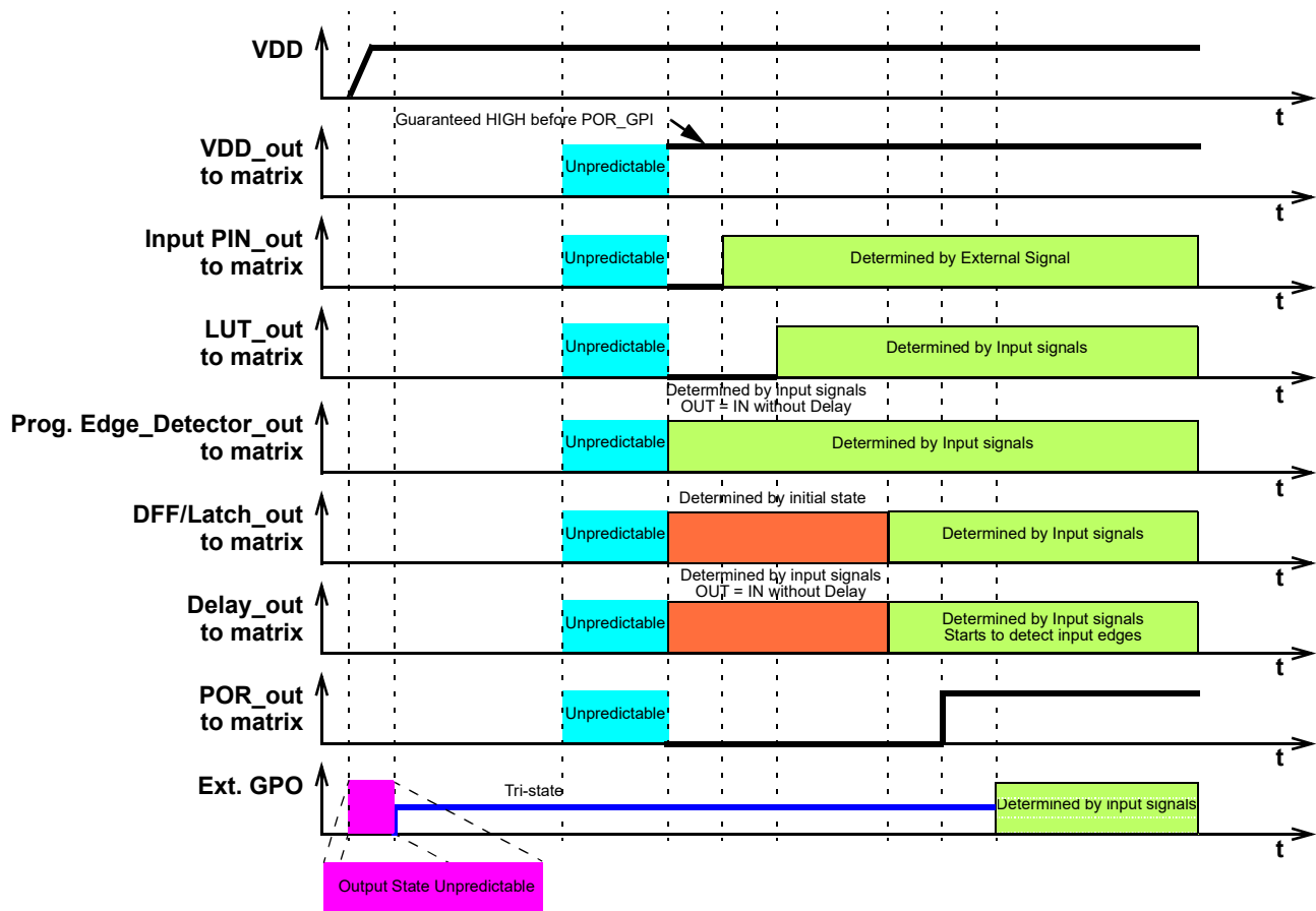
Figure 55. Internal Macrocell States during POR sequence
