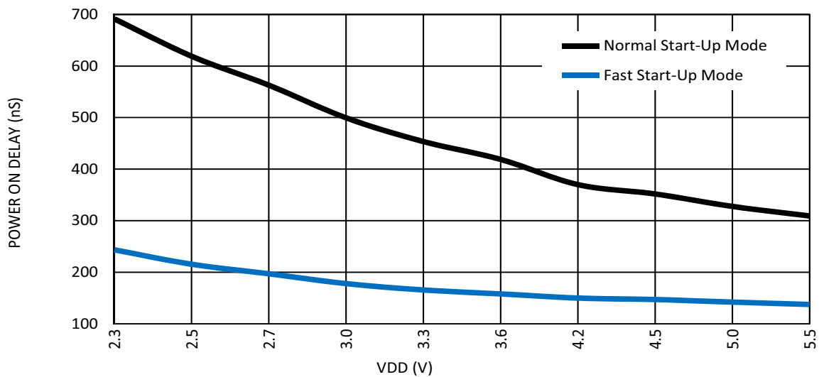
Figure 51. RC Oscillator Maximum Power On Delay vs. VDD at room temperature, OSC0 = 2 MHz
