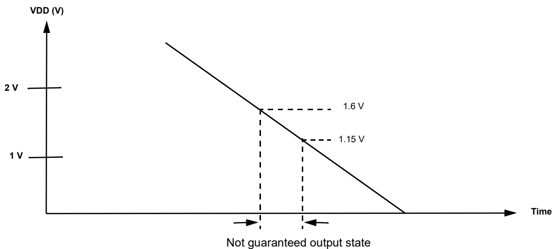
Figure 56. Power Down
