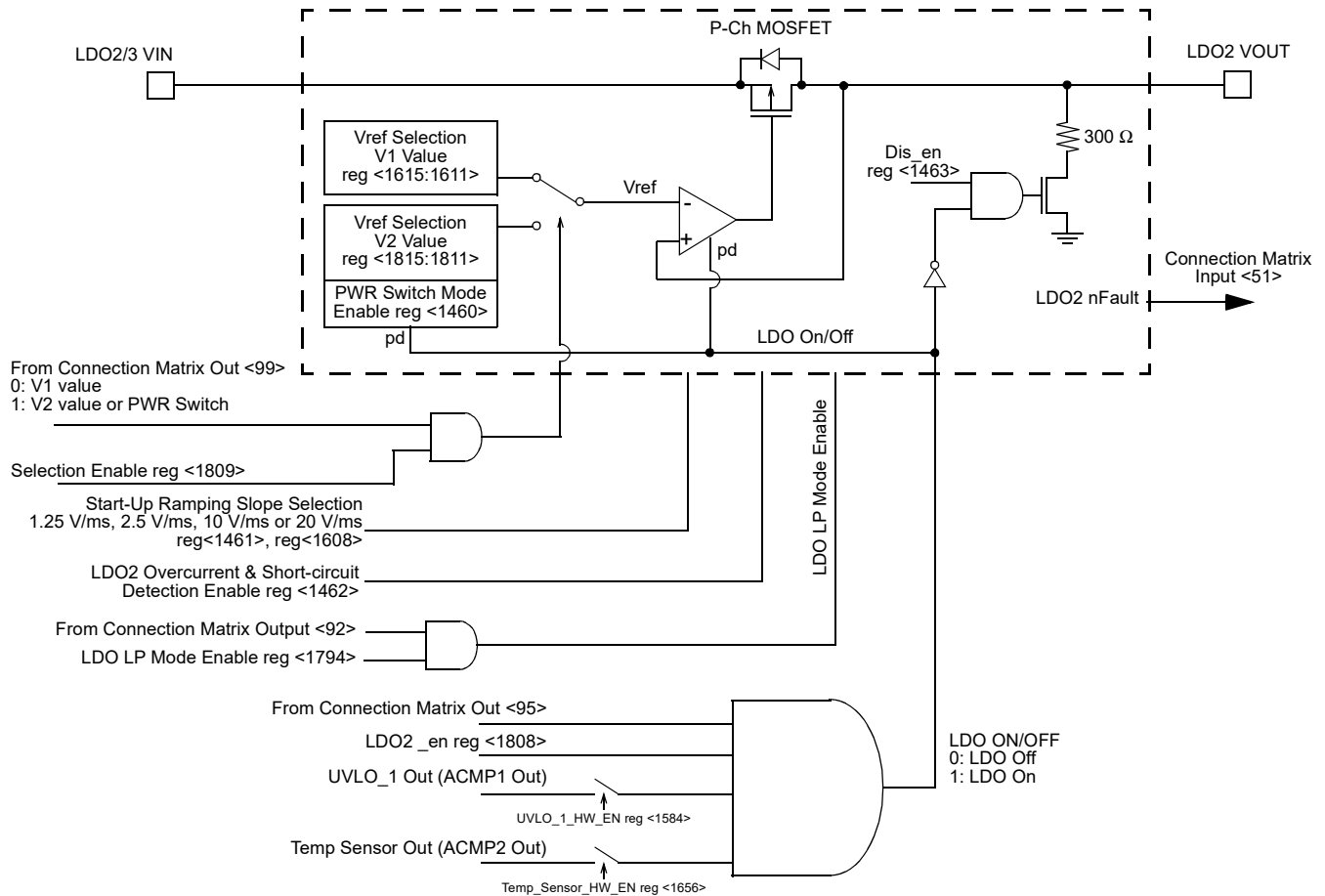
Figure 92. LDO2 Regulator Block Diagram
