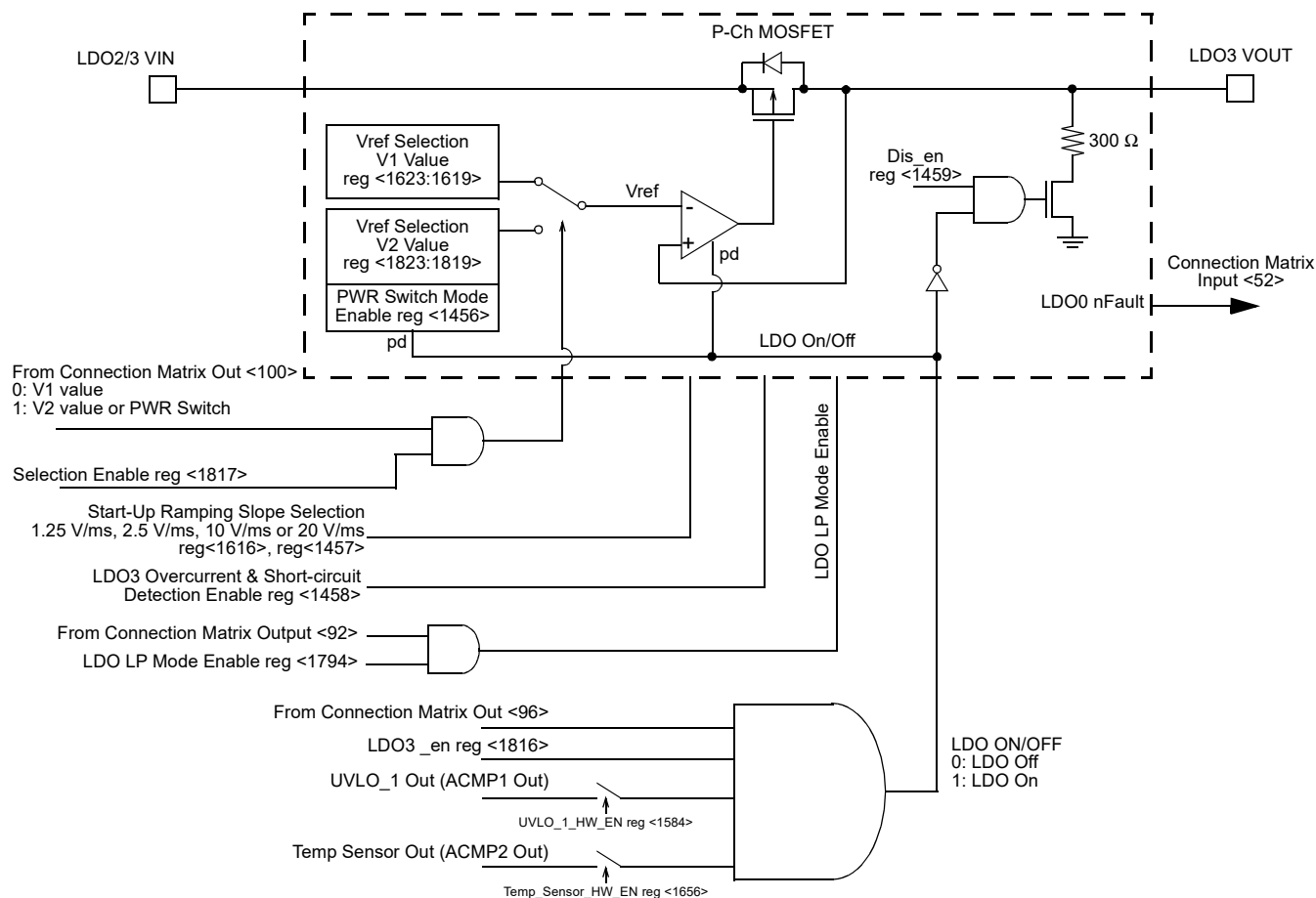
Figure 93. LDO3 Regulator Block Diagram
