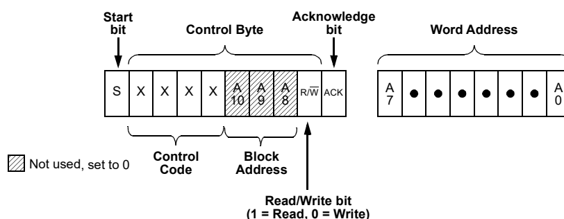
Figure 82. Basic Command Structure
