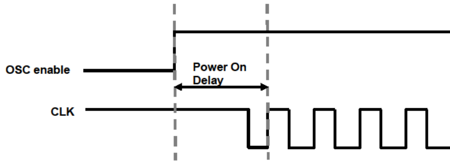
Figure 50. Oscillator Startup Diagram
