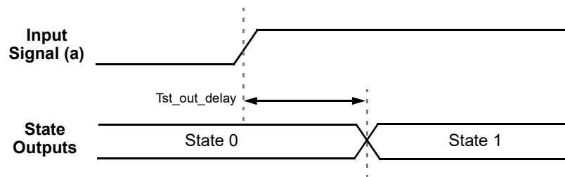
Figure 68. State Transition Timing
