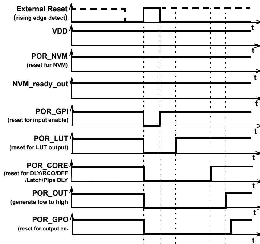
Figure 58. External reset sequence (Rising edge detect).
