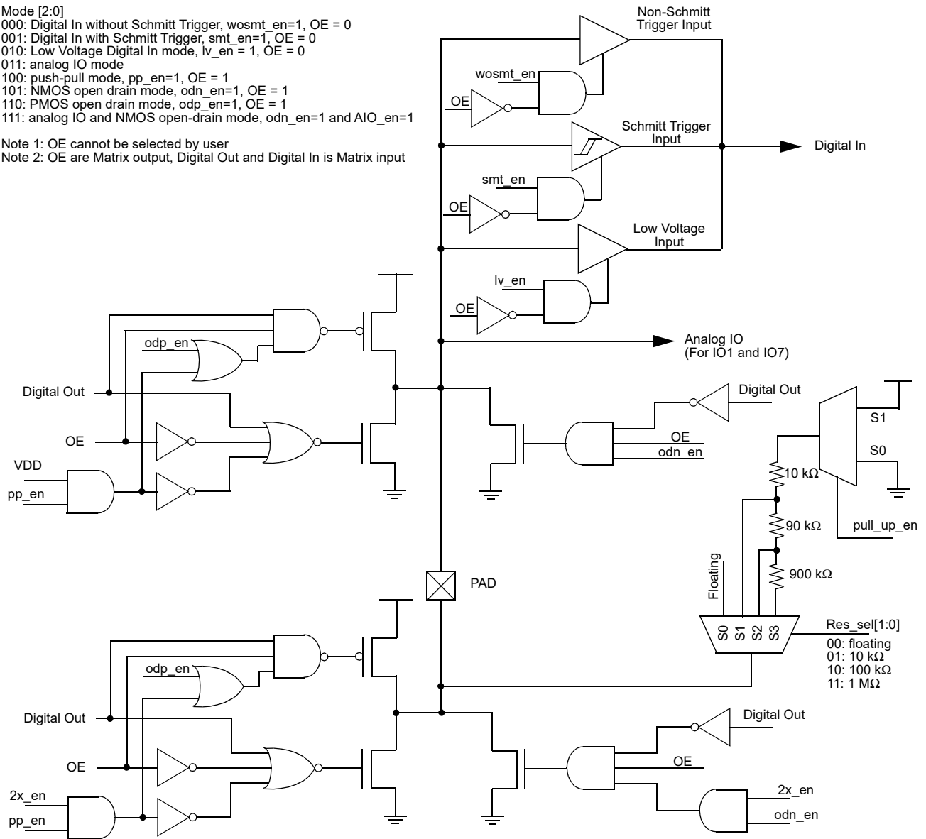
Figure 5. IO Structure Diagram
