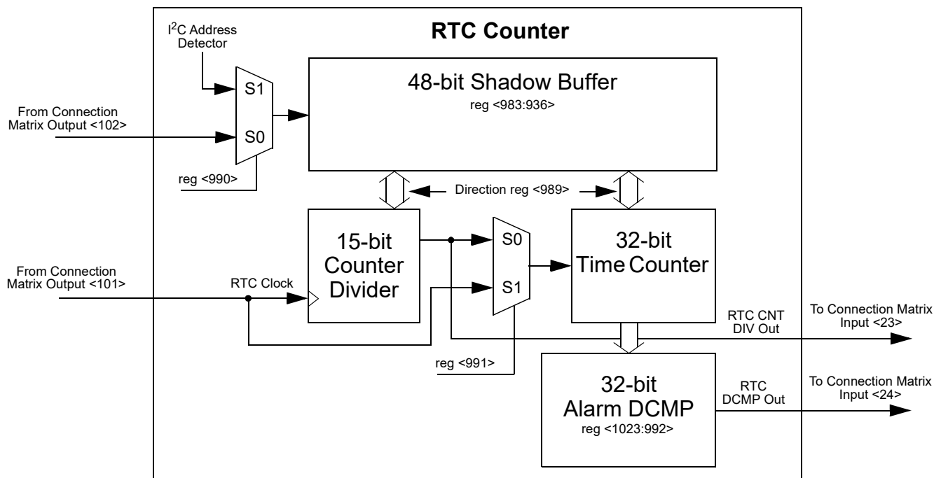
Figure 45. RTC Counter Macrocell
