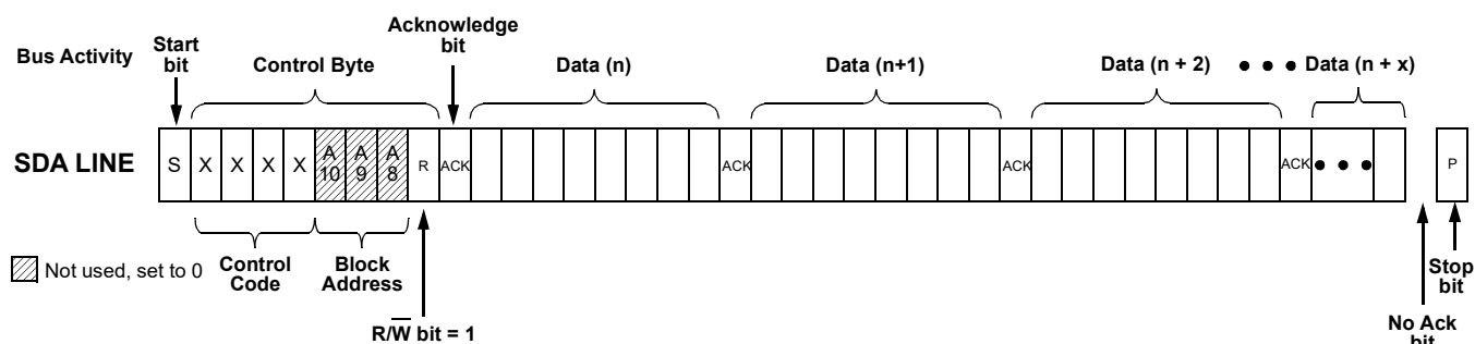
Figure 88. Sequential Read Command
