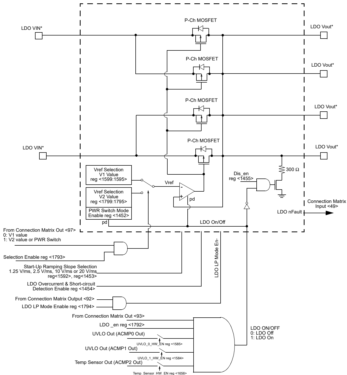
Figure 103. LDO Regulator Block Diagram
