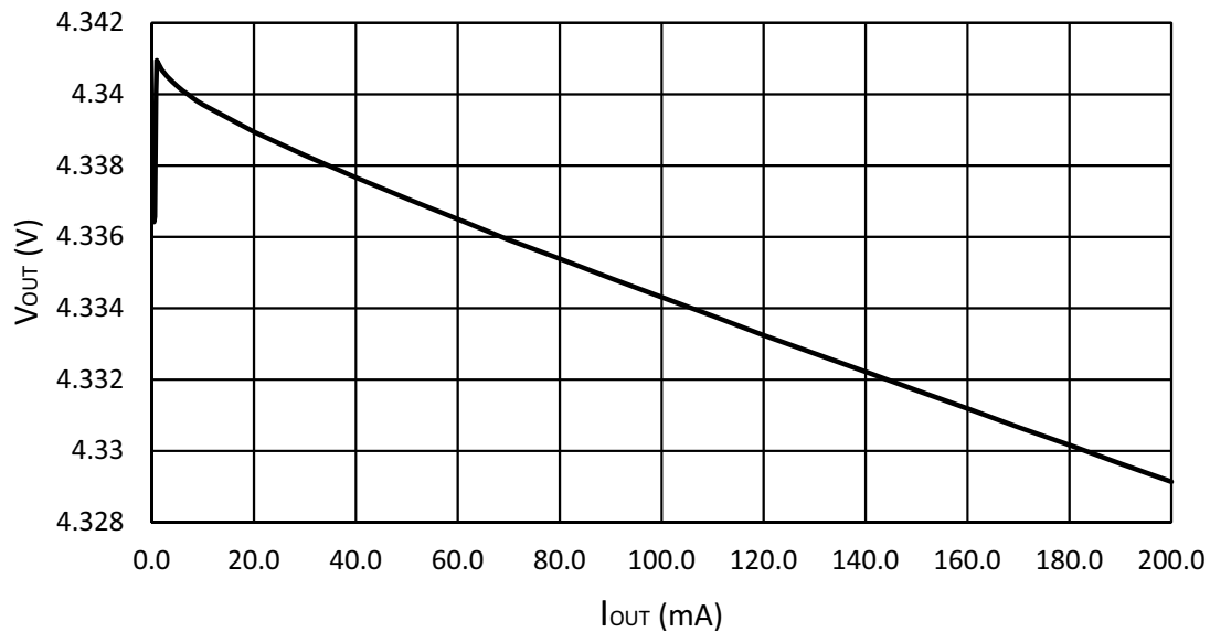
Figure 95. SLG46580 LDO Load Regulation, HIGH POWER Mode, T = 25°C, V DD = 5V, V OUT = 4.35 V
