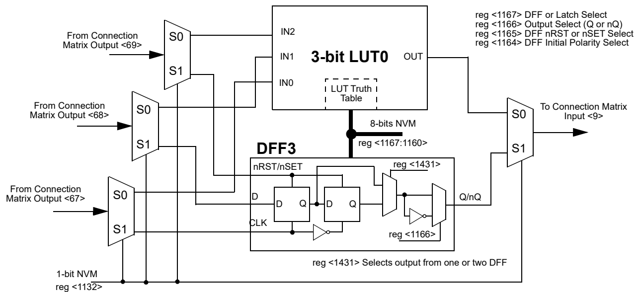
Figure 12. 3-bit LUT0 or DFF3
