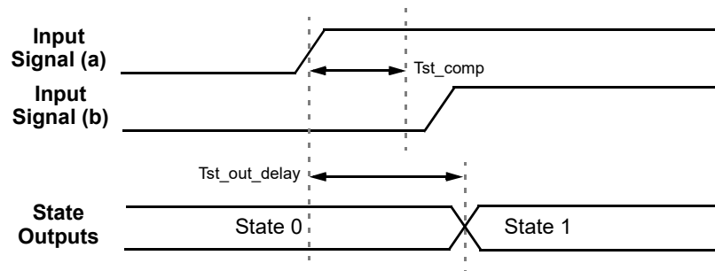
Figure 75. State Transition Timing - Competing Inputs Determinable
