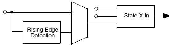
Figure 63. Rising Edge State Transition Selection (for each state X)
