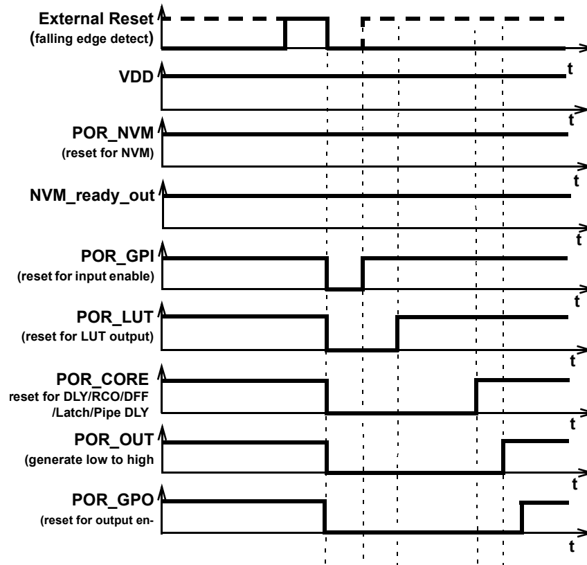
Figure 59. External reset sequence (Falling edge detect).
