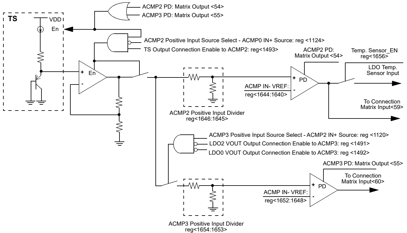
Figure 47. Analog Temperature Sensor Structure Diagram
