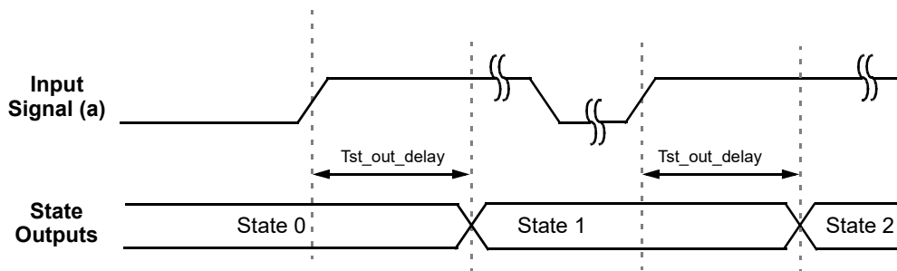
Figure 81. State Transition - Rising Edge Transition Timing
