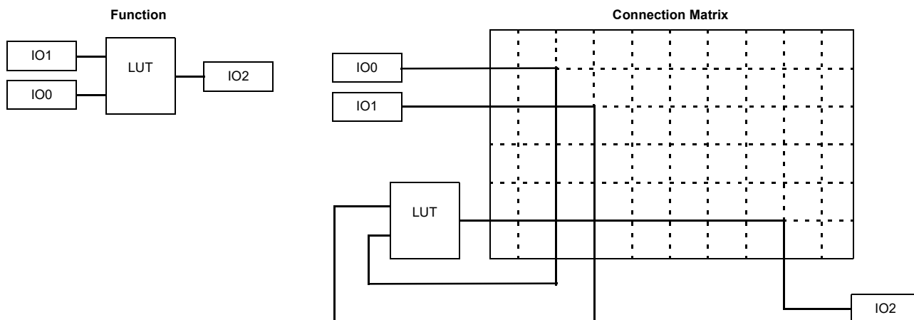
Figure 7. Connection Matrix Example
