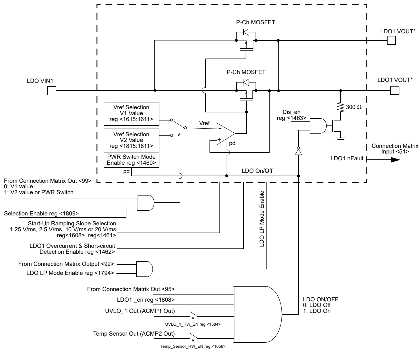
Figure 101. LDO1 Regulator Block Diagram
