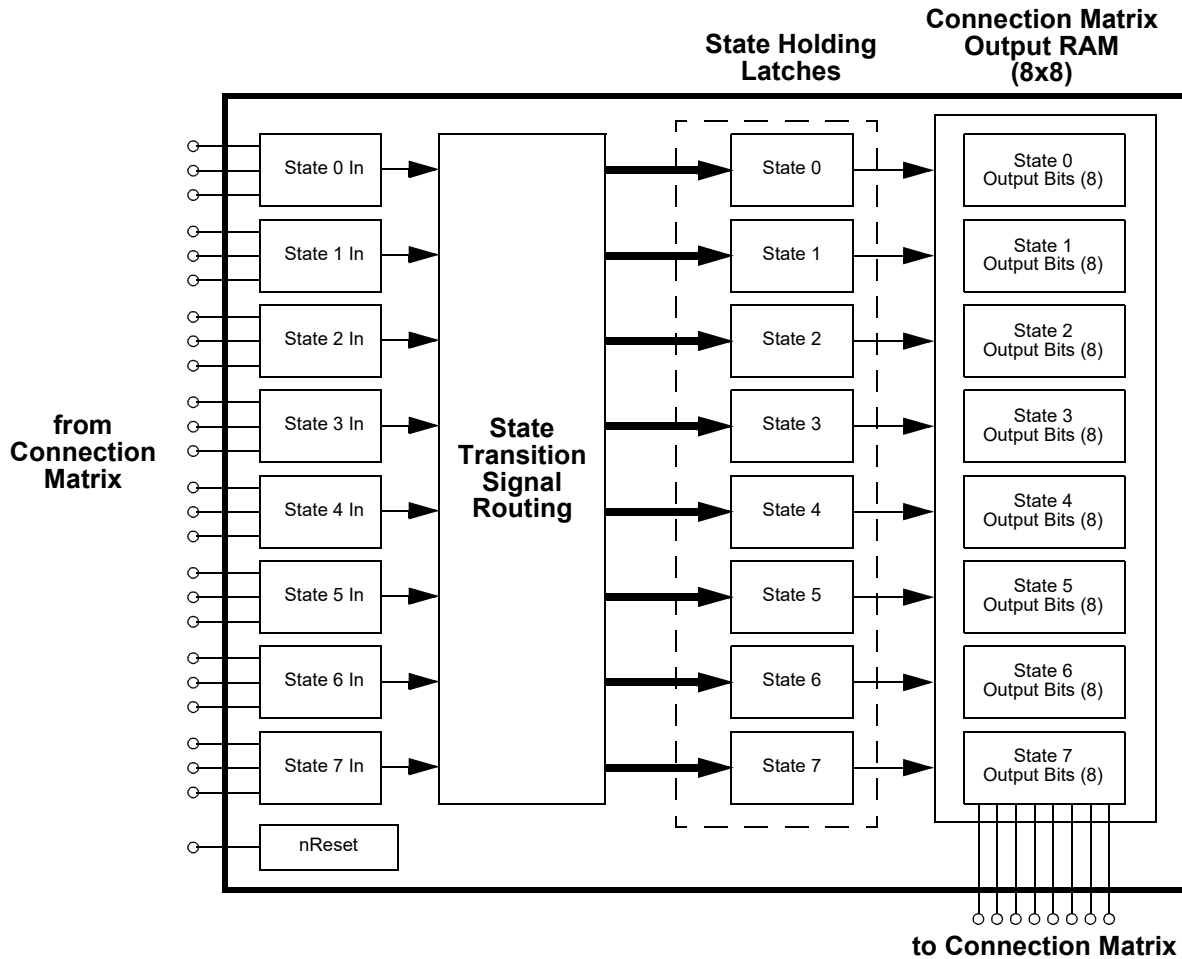
Figure 61. Asynchronous State Machine
