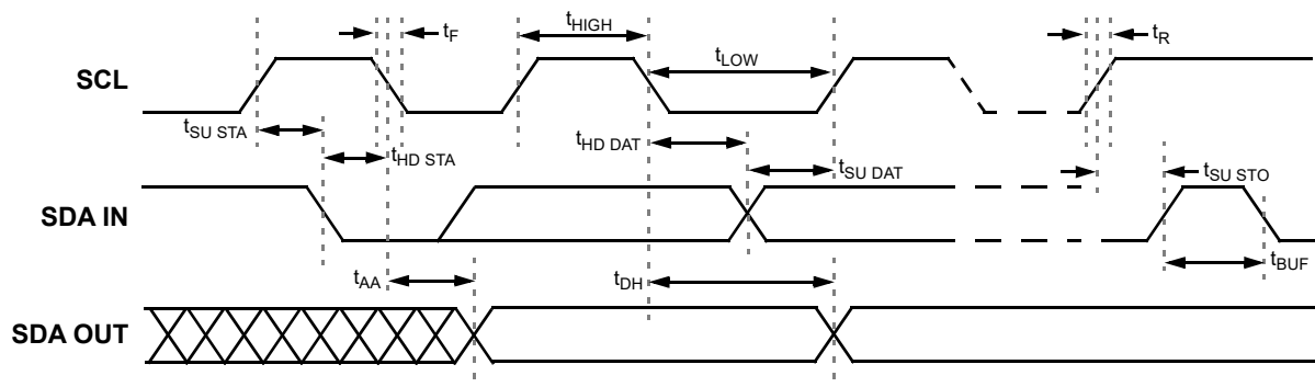
Figure 83. I 2 C General Timing Characteristics
