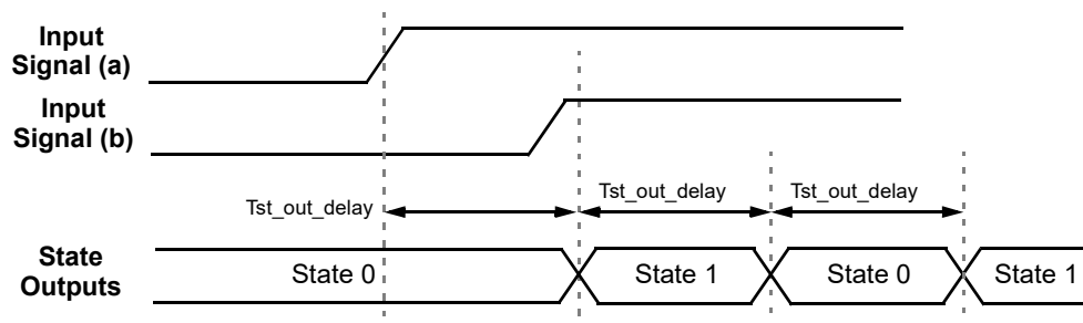
Figure 79. State Transition - Closed Cycling Timing
