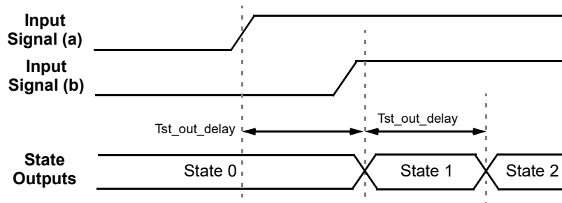
Figure 77. State Transition - Sequential Timing
