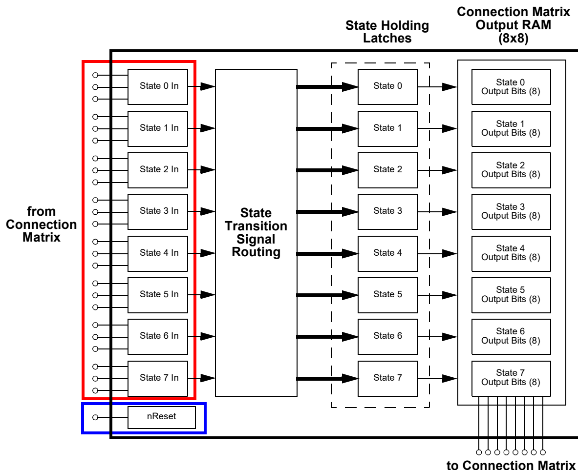
Figure 62. Asynchronous State Machine Inputs
