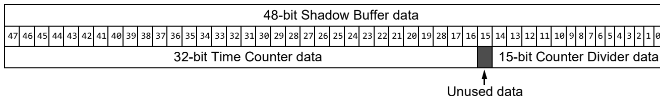
Figure 46. RTC Counter Shadow Buffer bits
