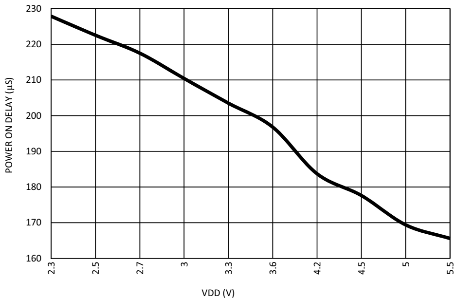
Figure 53. OSC1 (2 kHz) Maximum Power On Delay vs. VDD at 85°C
