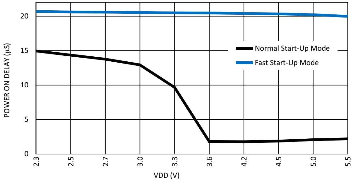
Figure 52. RC Oscillator Maximum Power On Delay vs. VDD at 85°C, OSC0 = 25 kHz
