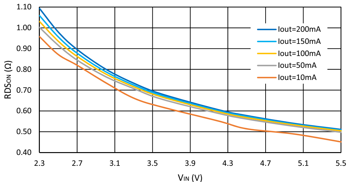
Figure 99. SLG46580 LDO P-channel ON resistance R DSon vs. V IN , Power Switch Mode, T = 25°C
