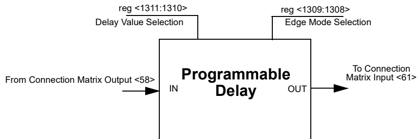
Figure 42. Programmable Delay
