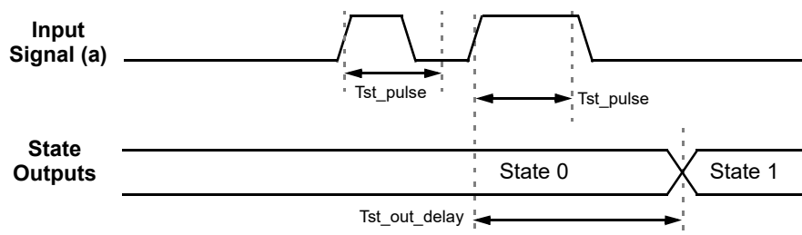
Figure 72. State Transition Pulse Input Timing
