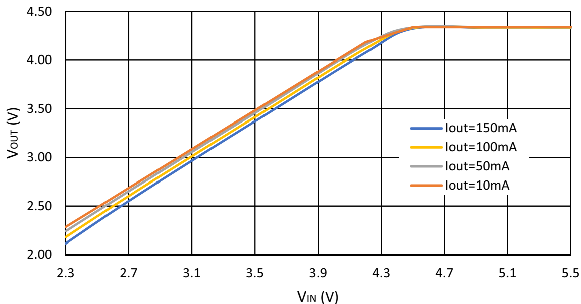
Figure 98. SLG46580 LDO High Power Mode V OUT vs. V IN , T = 25°C, V DD = 5V
