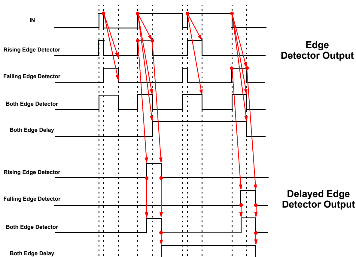
Figure 35. Glitch Filtering for Edge Detector Output
