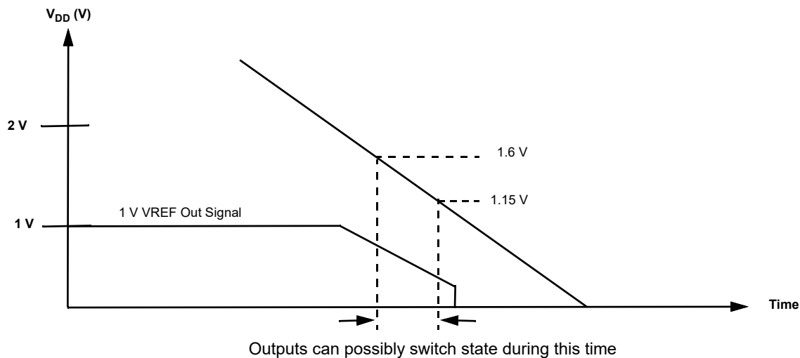
Figure 42. Power Down
