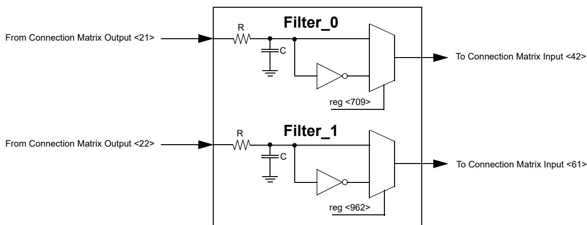
Figure 38. Deglitch Filter
