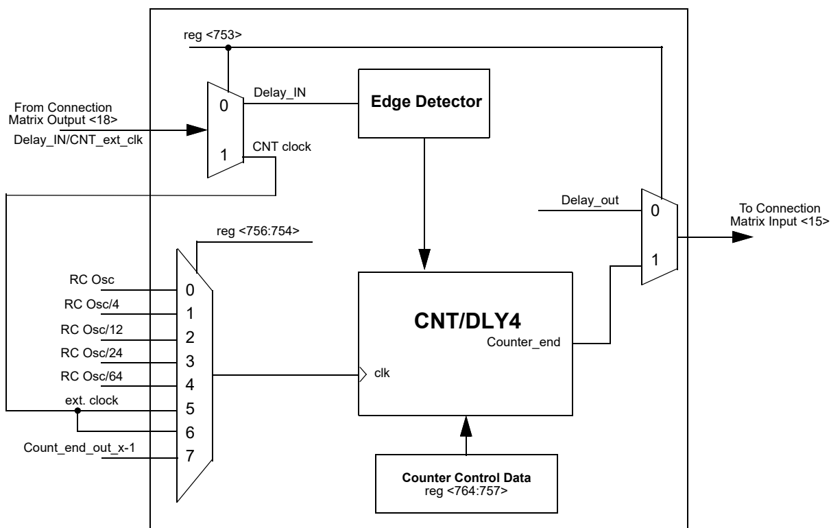
Figure 27. CNT/DLY4
