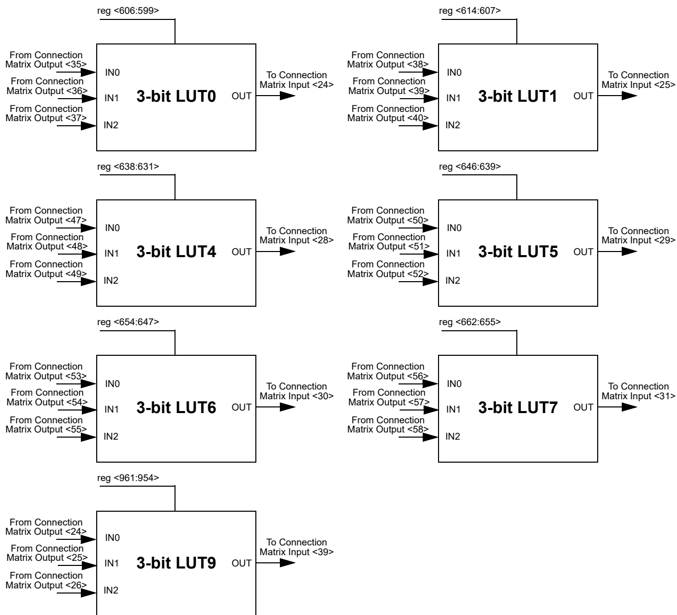
Figure 8. 3-bit LUTs
