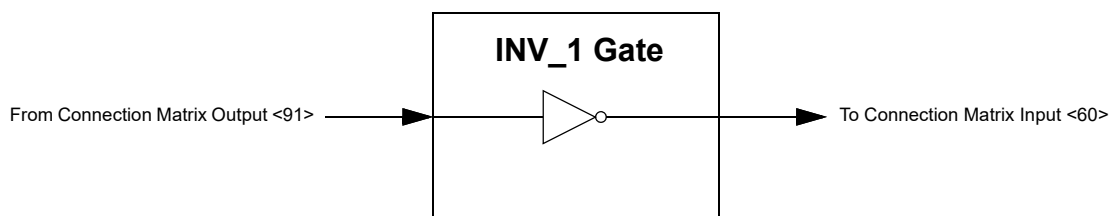
Figure 37. INV_1 Gate
