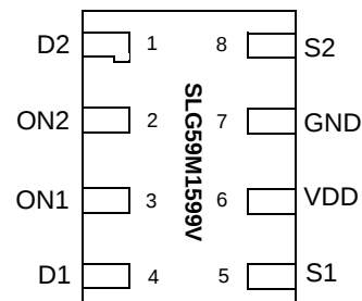
8-pin STDFN (Top View)
