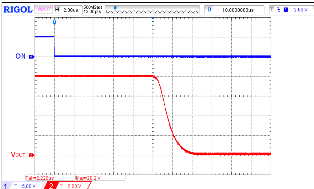
Figure 16. Typical Turn OFF operation waveform for V_{IN} = 20\text{ V} , C_{SLEW} = 10\text{ nF} , no C_{LOAD} , R_{LOAD} = 100\text{ Ω}
