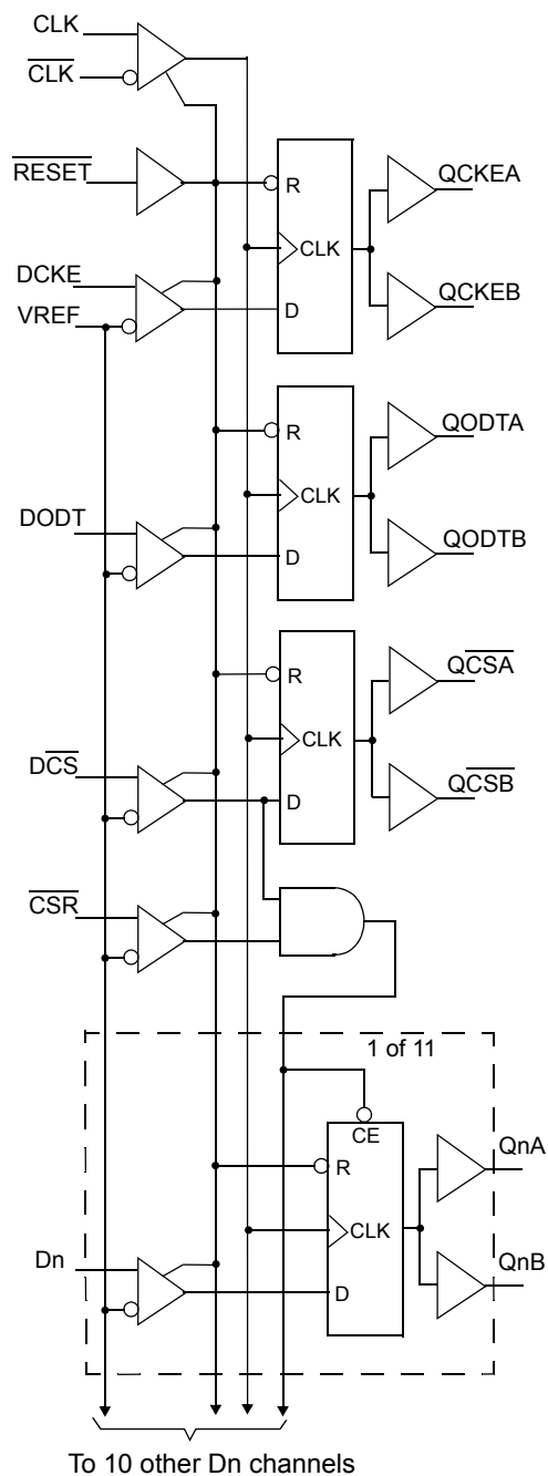
1:2 "B"- configuration Logic Diagram
