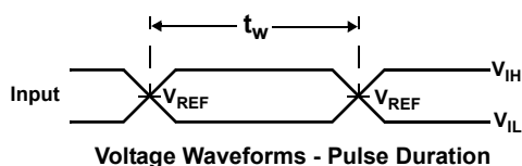
Voltage Waveforms - Pulse Duration
