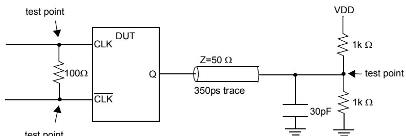
Output load test circuit
