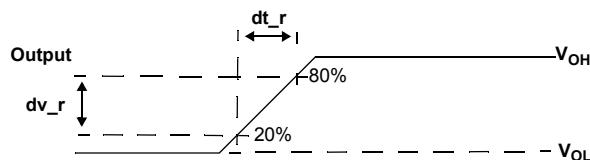
Voltage waveform: low to high slew rate
