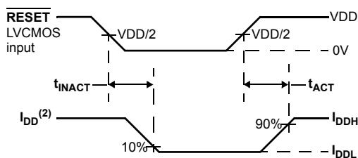
Voltage and Current Waveforms Inputs Active and Inactive Times
