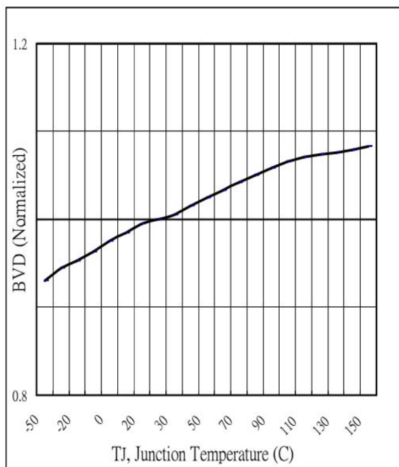
Fig.2 Breakdown Voltage Variation vs. Temperature
