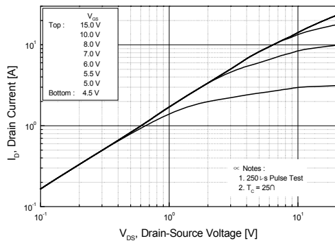
Figure 1. On-Region Characteristics
