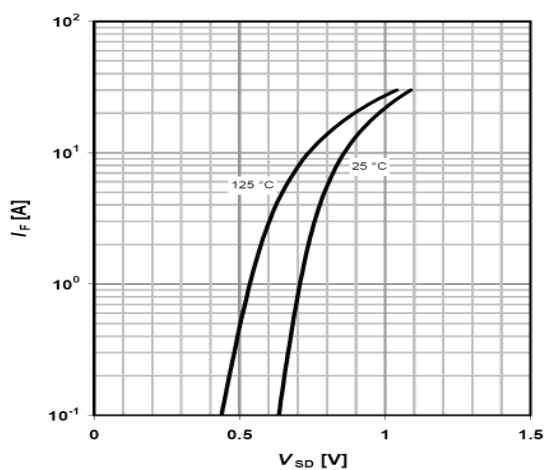
Figure 7: Body-Diode Characteristics
