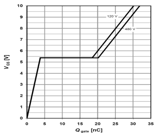
Figure 8: Gate-Charge Characteristics
