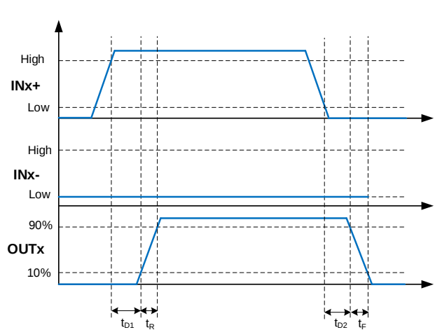
Figure 3. Non-Inverting Input Driver Operation
