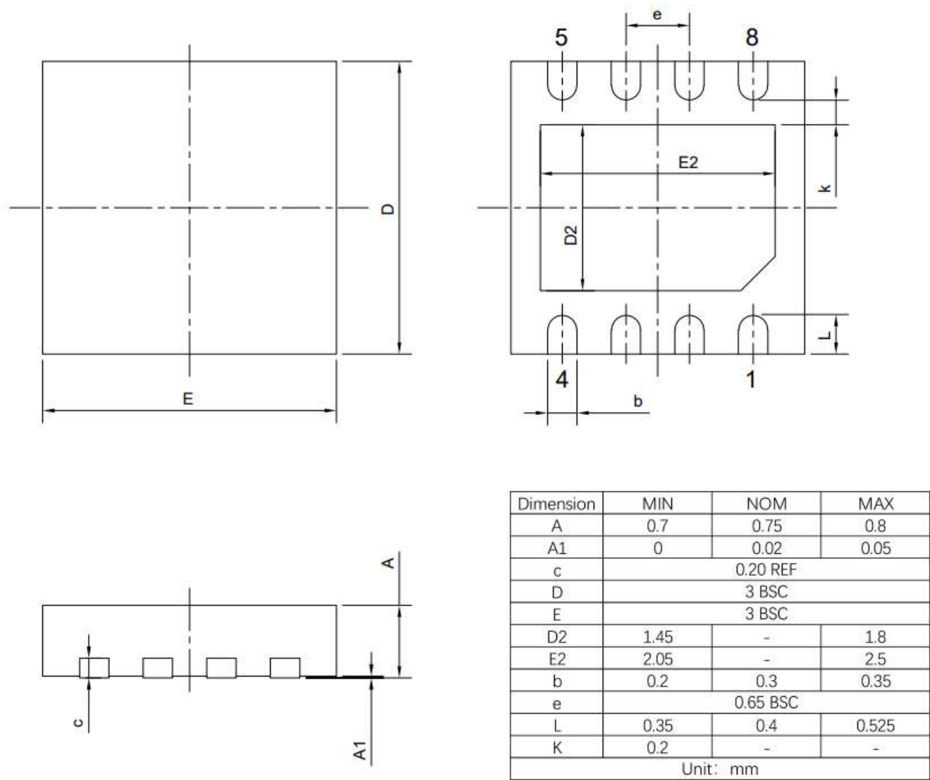
Figure 5. Package Outline Dimensions
