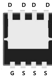
DFN3*3
