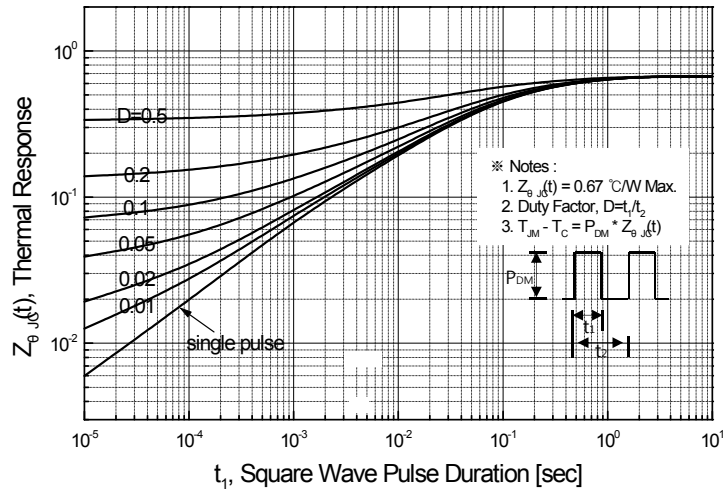
Figure 11-1. Transient Thermal Response Curve for SLP10N60C
