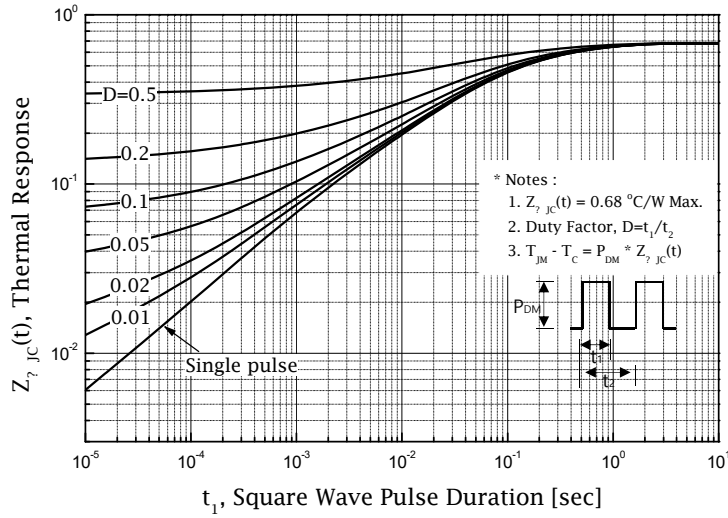
Figure 11-1. Transient Thermal Response Curve for SLP10N60U
