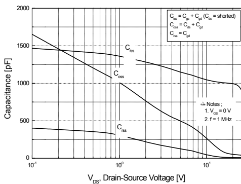
Figure 5. Capacitance Characteristics
