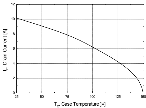
Figure 10. Maximum Drain Current
