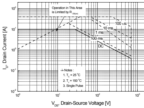
Figure 9-1. Maximum Safe Operating Area for SLP10N70C
