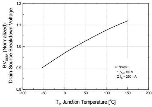
Figure 7. Breakdown Voltage Variation
