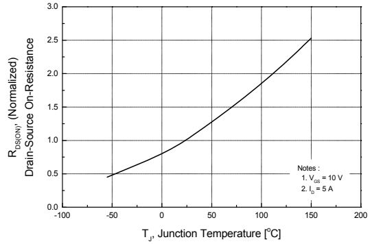
Figure 8. On-Resistance Variation
