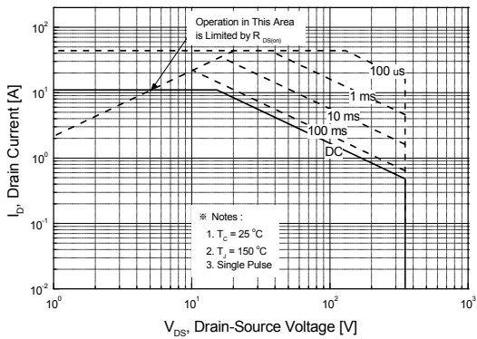
Figure 9-1. Maximum Safe Operating Area for SLP11N35UZ
