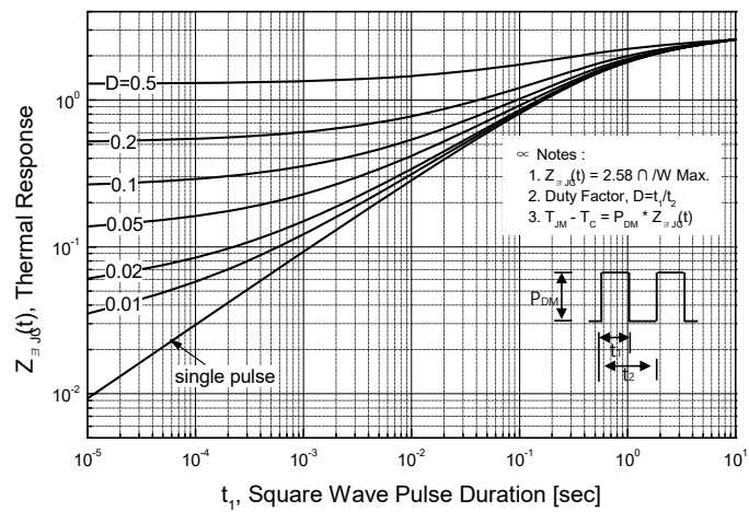
Figure 11-2. Transient Thermal Response Curve for SLF14N50C
