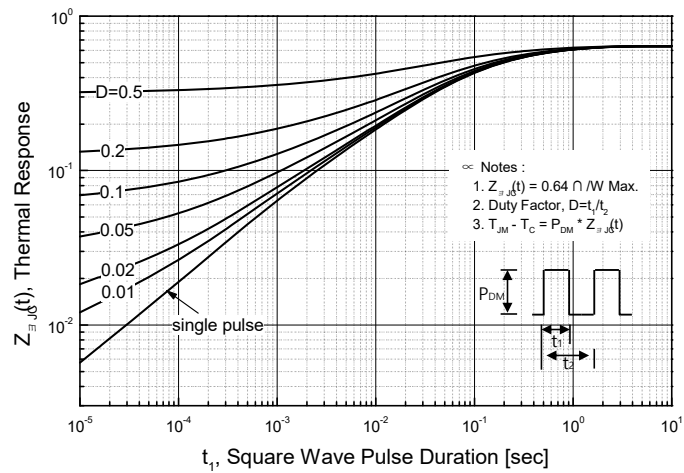
Figure 11-1. Transient Thermal Response Curve for SLP14N50C
