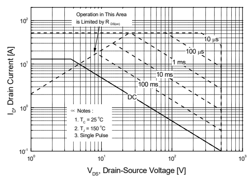
Figure 9-2. Maximum Safe Operating Area for SLF14N50C
