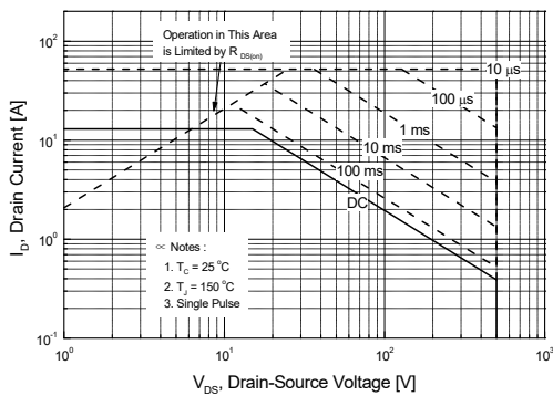
Figure 9-1. Maximum Safe Operating Area for SLP14N50C
