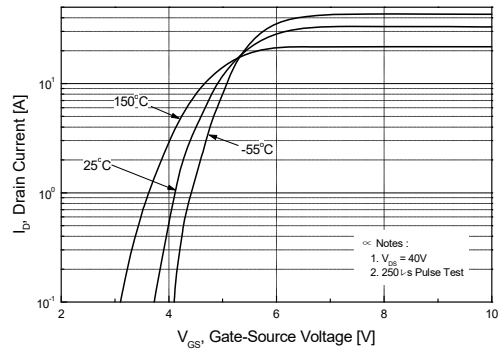
Figure 2. Transfer Characteristics
