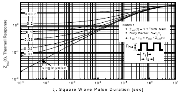
Figure 11-2. Transient Thermal Response Curve for SLF2N60C
