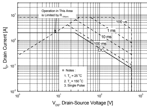
Figure 9-1. Maximum Safe Operating Area For SLP2N60UZ
