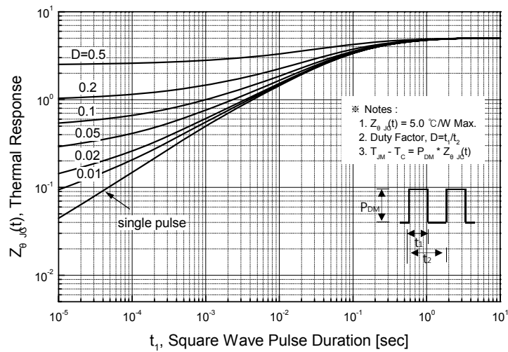
Figure 11-2. Transient Thermal Response Curve for SLF2N60UZ
