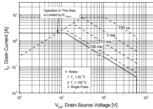
Figure 9-2. Maximum Safe Operating Area For SLF2N60UZ
