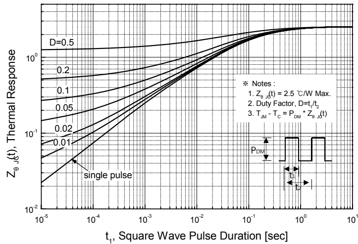
Figure 11-1. Transient Thermal Response Curve for SLP2N60UZ
