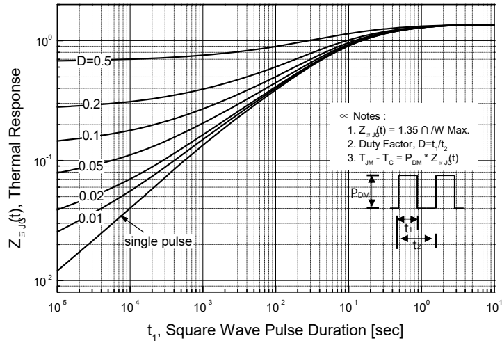
Figure 11-1. Transient Thermal Response Curve for SLP4N60C
