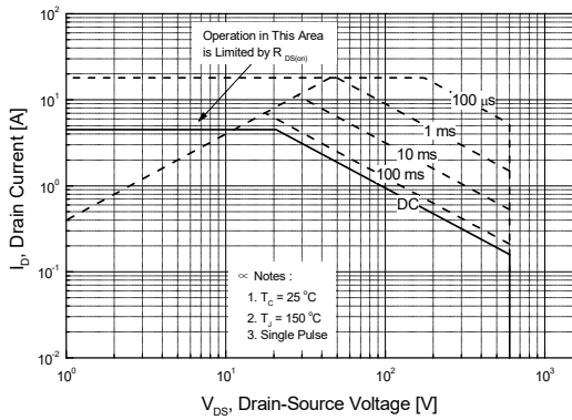
Figure 9-1. Maximum Safe Operating Area for SLP4N60C
