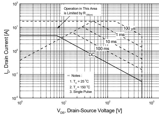
Figure 9-2. Maximum Safe Operating Area for SLF4N60C
