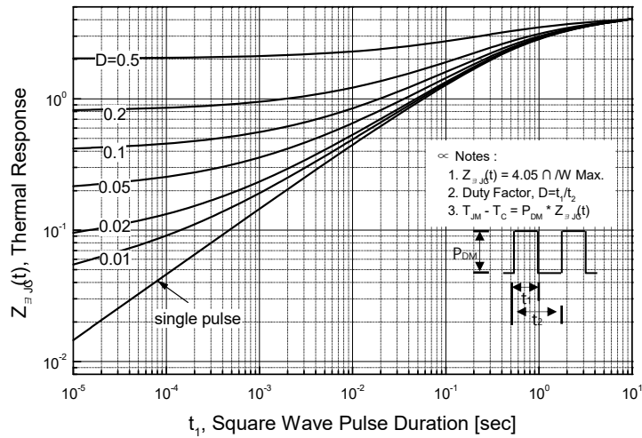
Figure 11-2. Transient Thermal Response Curve for SLF4N60C
