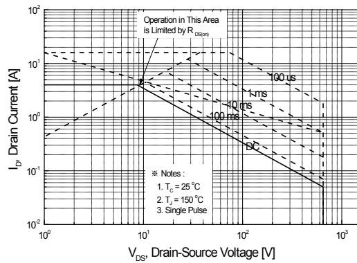
Figure 9-2. Maximum Safe Operating Area for SLF4N65UZ
