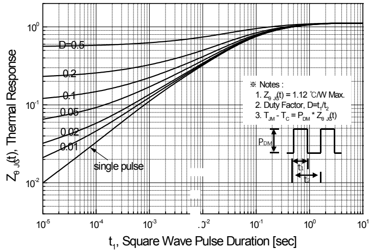
Figure 11-1. Transient Thermal Response Curve for SLP4N65UZ
