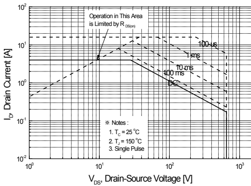
Figure 9-1. Maximum Safe Operating Area for SLP4N65UZ
