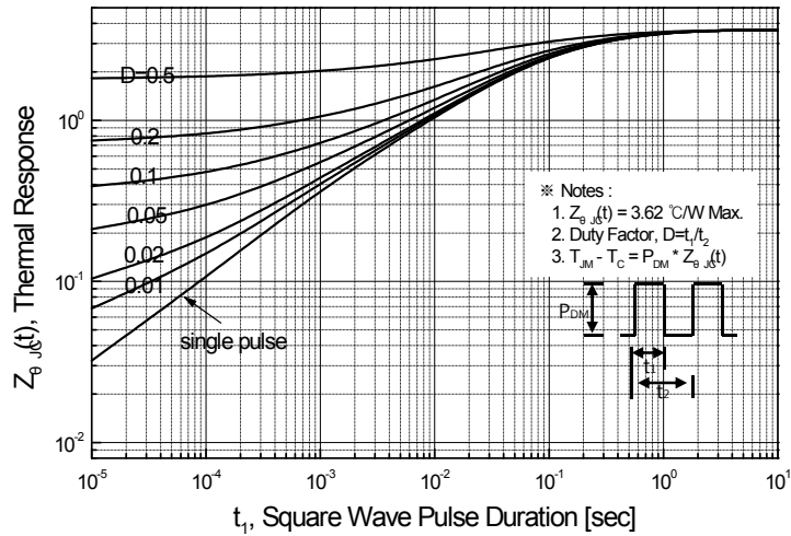
Figure 11-2. Transient Thermal Response Curve for SLF4N65UZ
