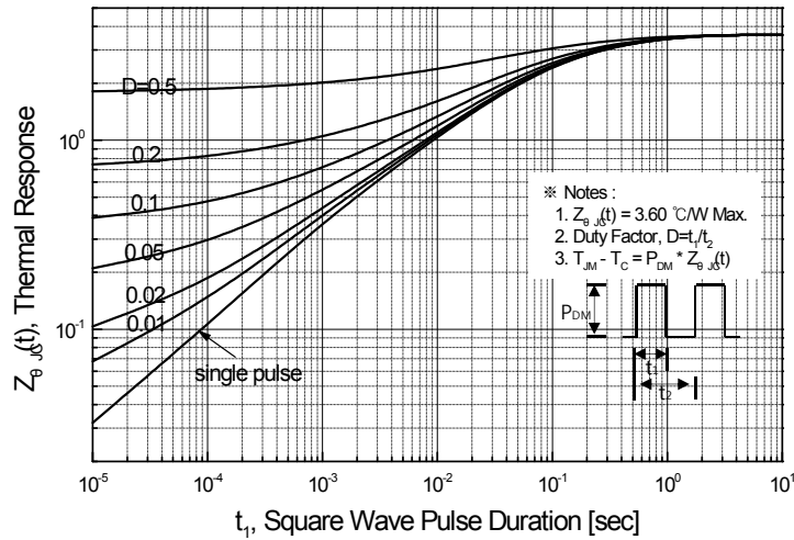
Figure 11-2. Transient Thermal Response Curve for SLF4N70C
