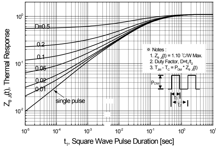
Figure 11-1. Transient Thermal Response Curve for SLP4N70C
