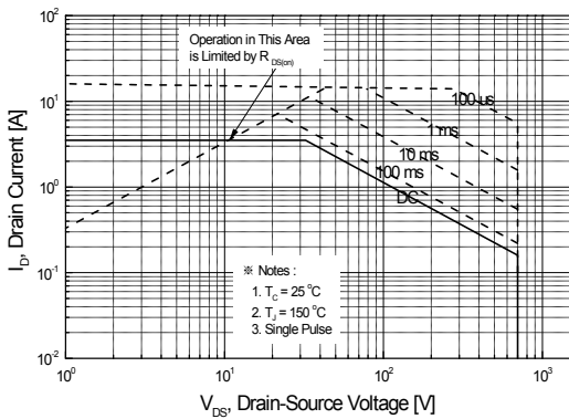
Figure 9-1. Maximum Safe Operating Area for SLP4N70C
