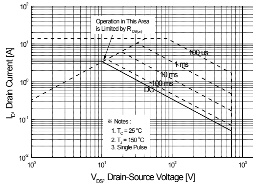
Figure 9-2. Maximum Safe Operating Area for SLF4N70C
