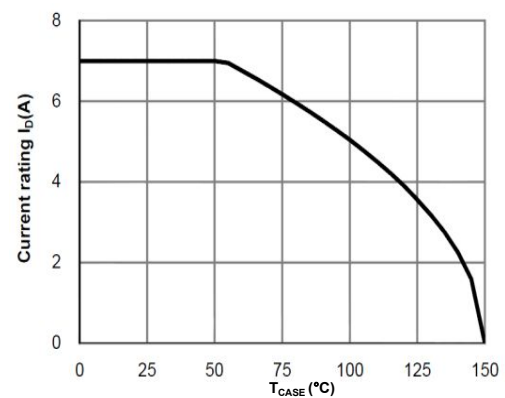
Figure 14: Current De-rating
