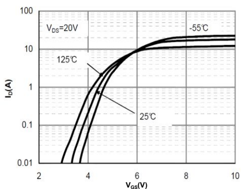
Figure 3: Transfer Characteristics
