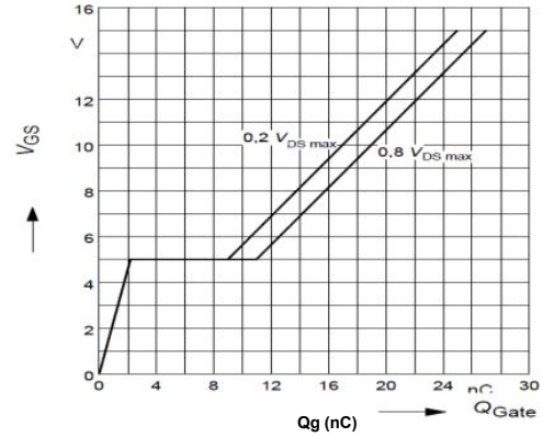
Figure 8: Gate-Charge Characteristics
