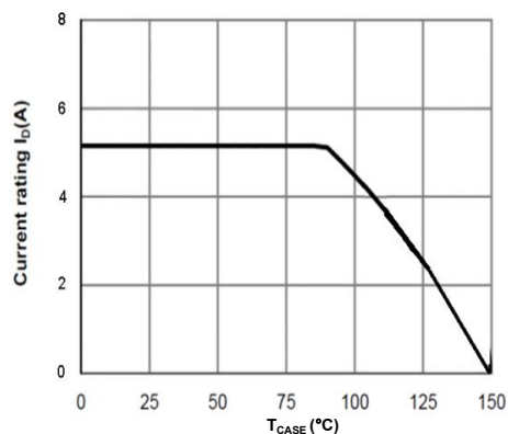
Figure 15: Current De-rating
