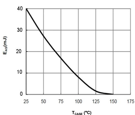
Figure 14: Avalanche energy
