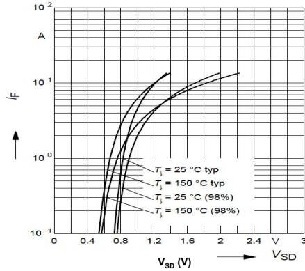
Figure 7: Body-Diode Characteristics
