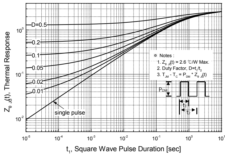
Figure 11-2. Transient Thermal Response Curve for SLF6N70U
