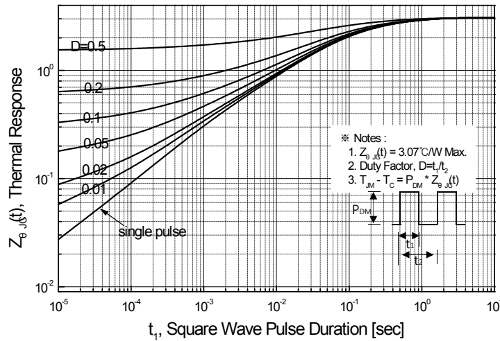
Figure 11-2. Transient Thermal Response Curve For TO-220F
