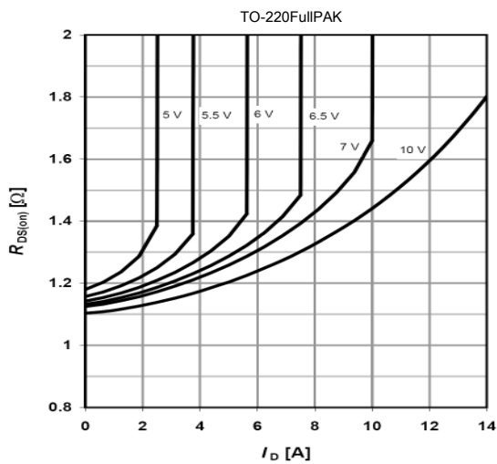
Figure 6: On-Resistance vs. Drain Current, T_j=125^\circ\text{C}
