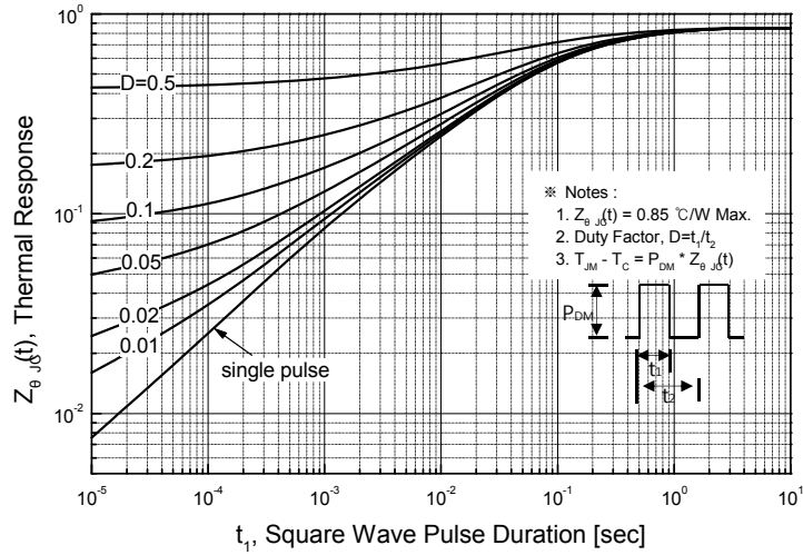
Figure 11-1. Transient Thermal Response Curve for SLP8N65U
