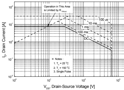
Figure 9-1. Maximum Safe Operating Area for SLP8N65U
