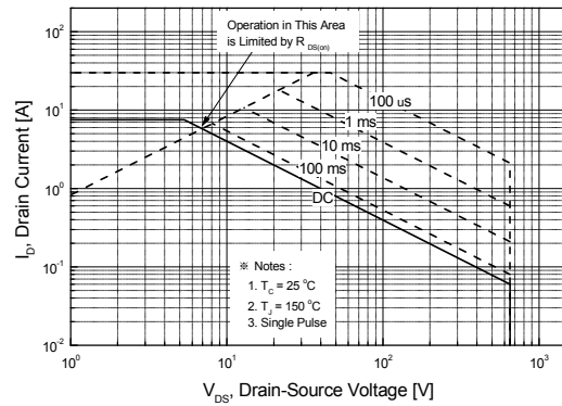
Figure 9-2. Maximum Safe Operating Area for SLF8N65U
