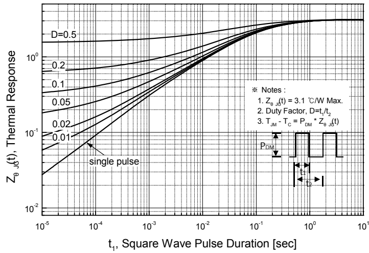
Figure 11-2. Transient Thermal Response Curve for SLF8N65U
