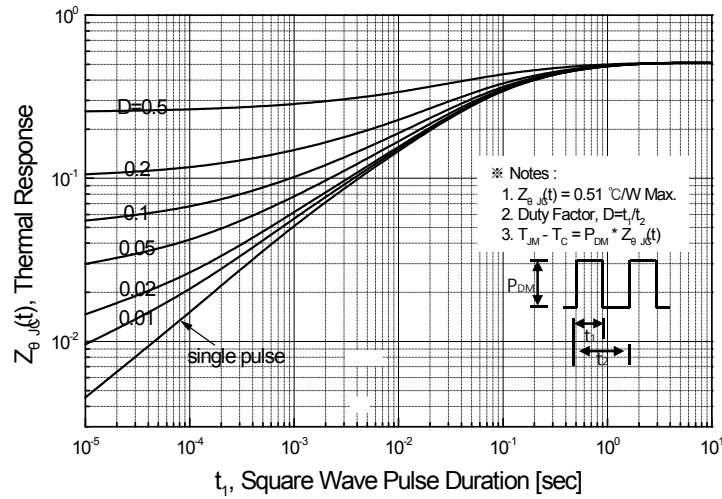
Figure 11. Transient Thermal Response Curve for SLP9N90CZ
