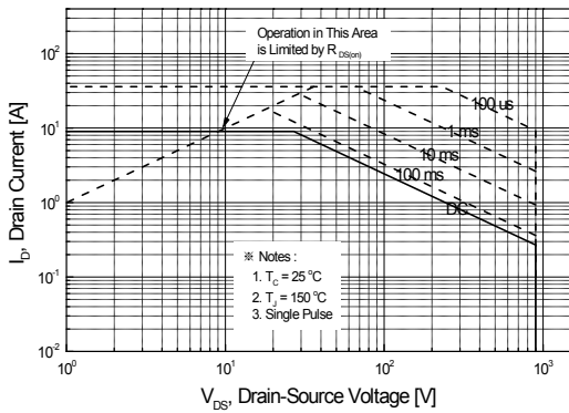
Figure 9. Maximum Safe Operating Area for SLP9N90CZ
