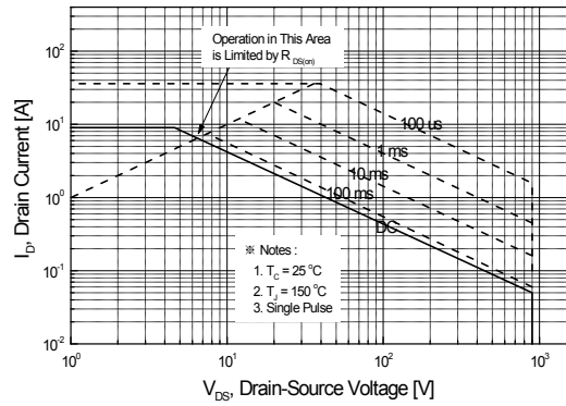
Figure 9. Maximum Safe Operating Area for SLF9N90CZ
