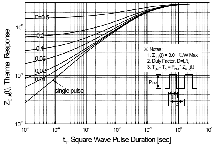
Figure 11. Transient Thermal Response Curve for SLF9N90CZ
