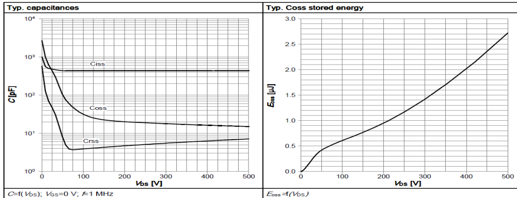
Figure 13: Capacitances
